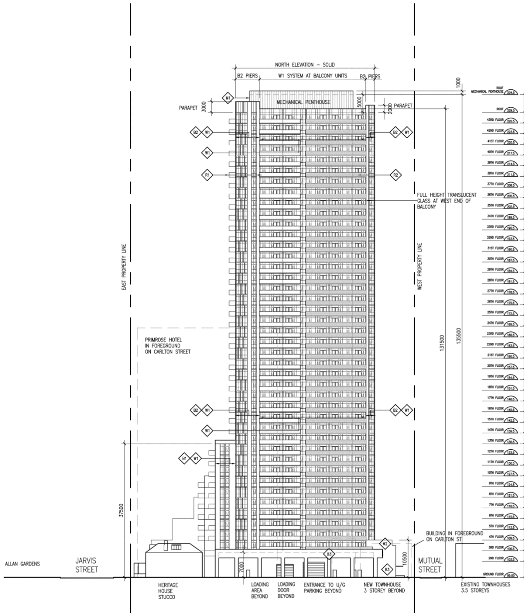
North Elevation
