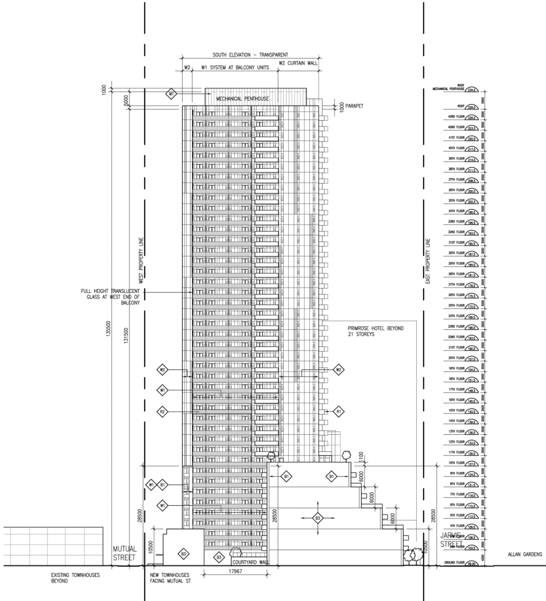
South Elevation
