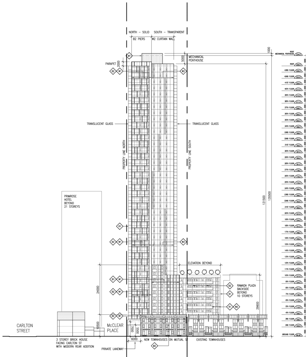
West Elevation
