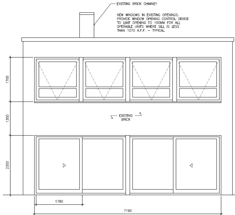
Proposed South (Rear) Elevation
