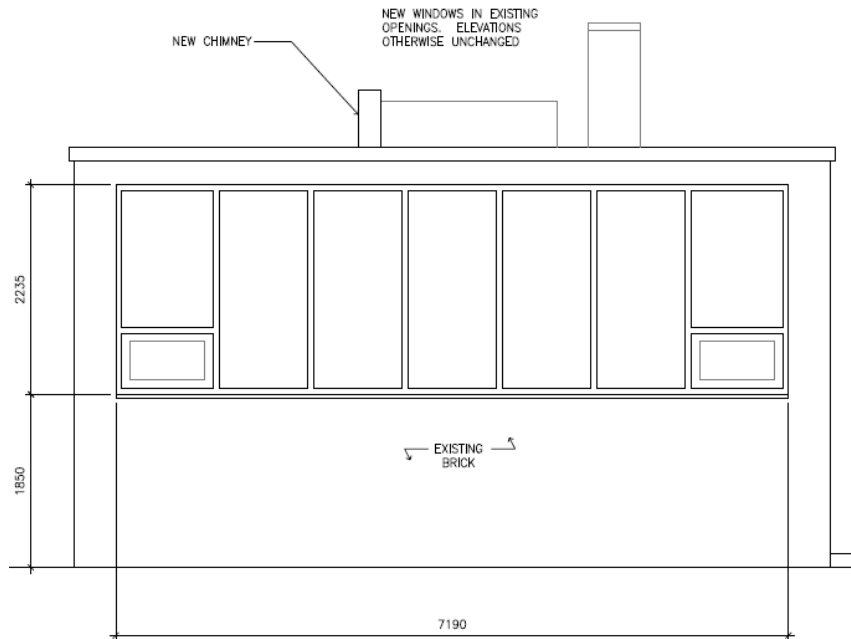
Proposed North (Front) Elevation
