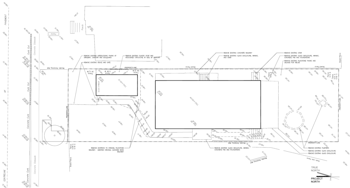
Existing Site Plan
