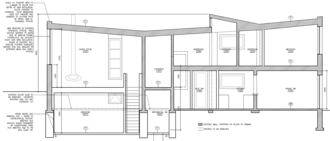
Proposed Building Section
