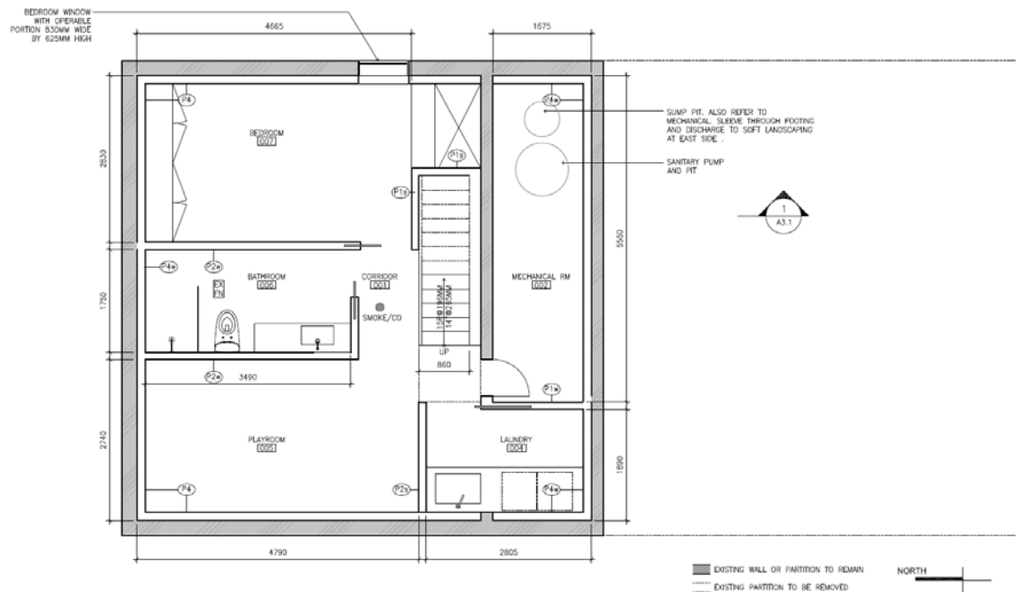
Proposed Basement Plan
