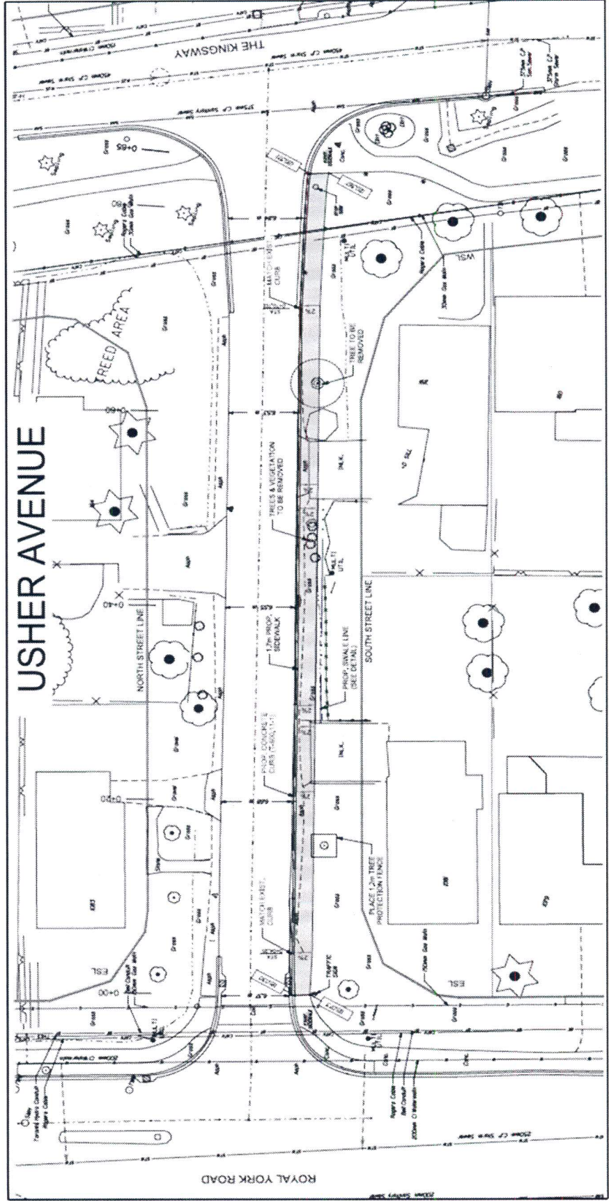
Appendix 1: Usher Avenue from Royal York Road to the Kingsway – Sidewalk Construction Plan and Profile
