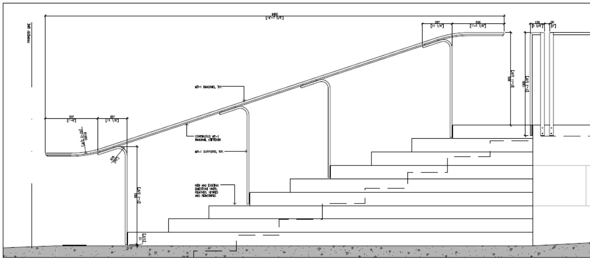
Proposed Elevation of Main Stair Handrail
