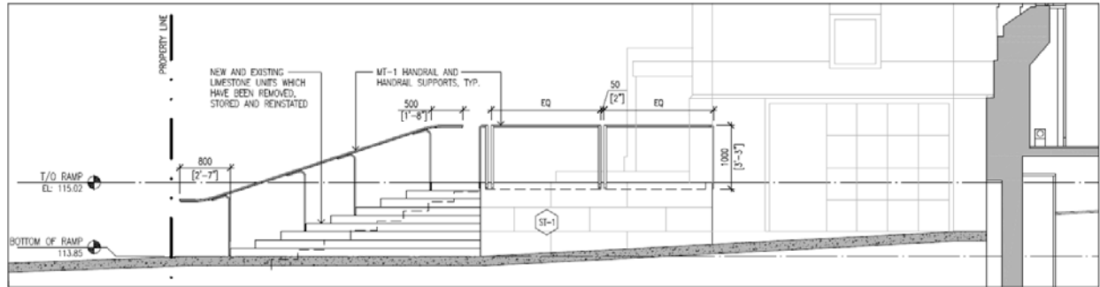
Proposed North Elevation at East Entrance
