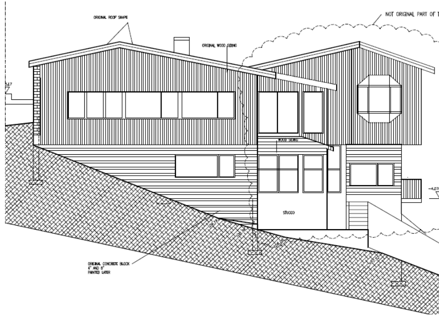
Existing West (rear) Elevation
