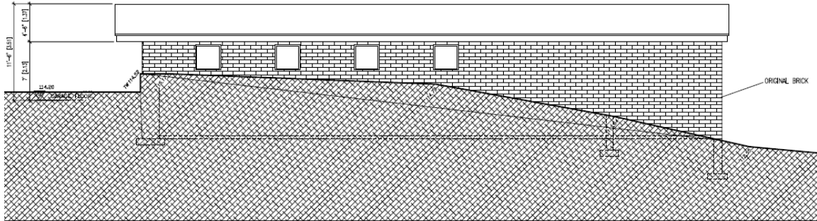
Existing North Elevation
