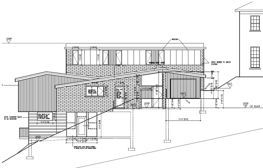
Proposed Primary (East) Elevation
