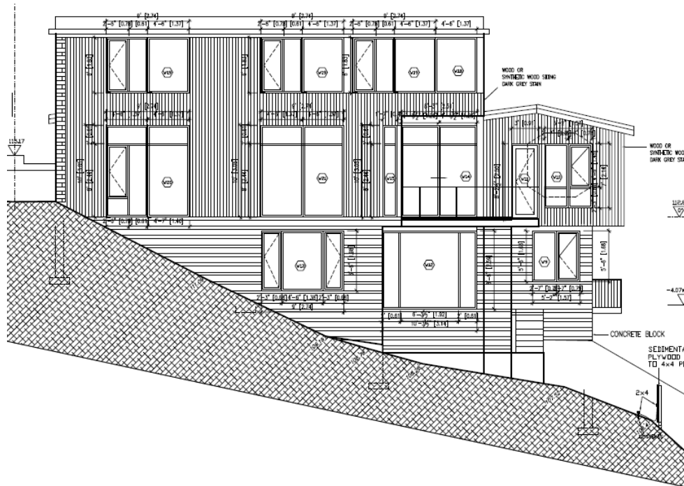
Proposed West (rear) Elevation
