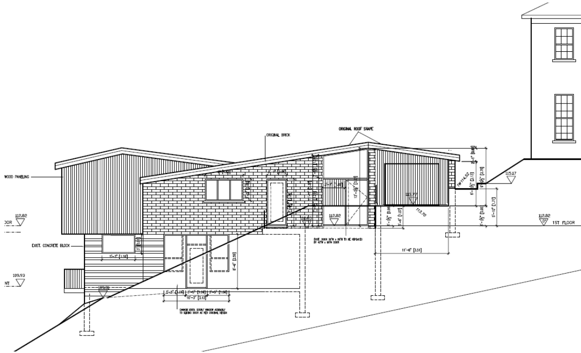
Existing Primary (East) Elevation
