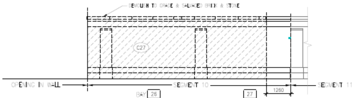
Segment 10 - East Elevation
