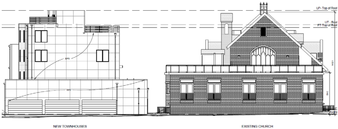
Proposed East (Rear) Elevation – 169 & 175 Jones Avenue
