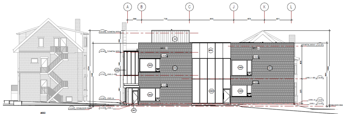
East (Rear) Elevation
