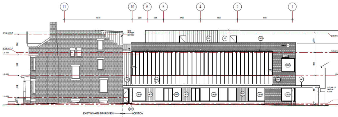
North (Side) Elevation
