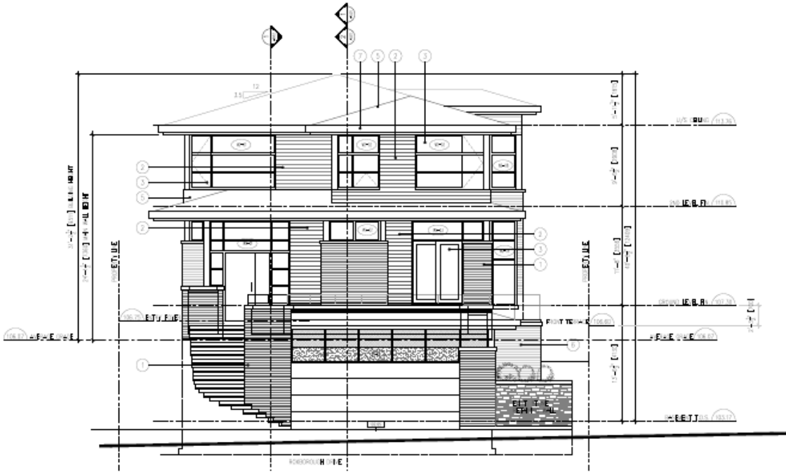
Primary (South) Elevation
