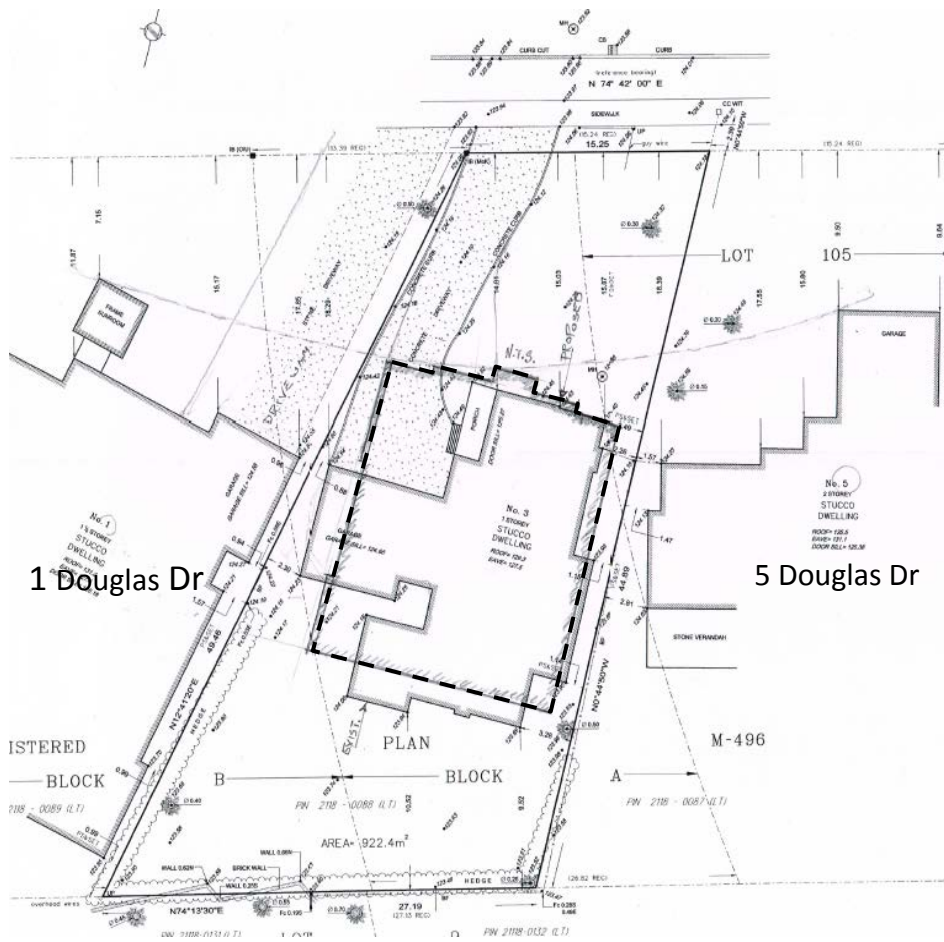
Site Plan showing existing house with footprint of new house shown in dashed line
