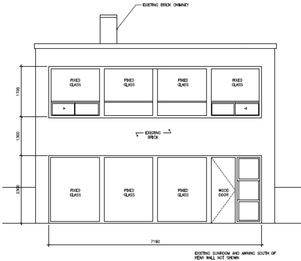
Existing South (Rear) Elevation
