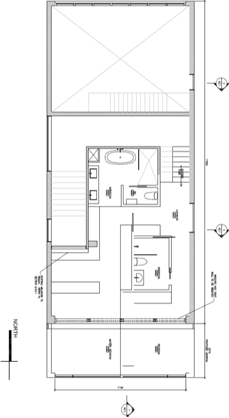
Proposed Upper Floor Plan
