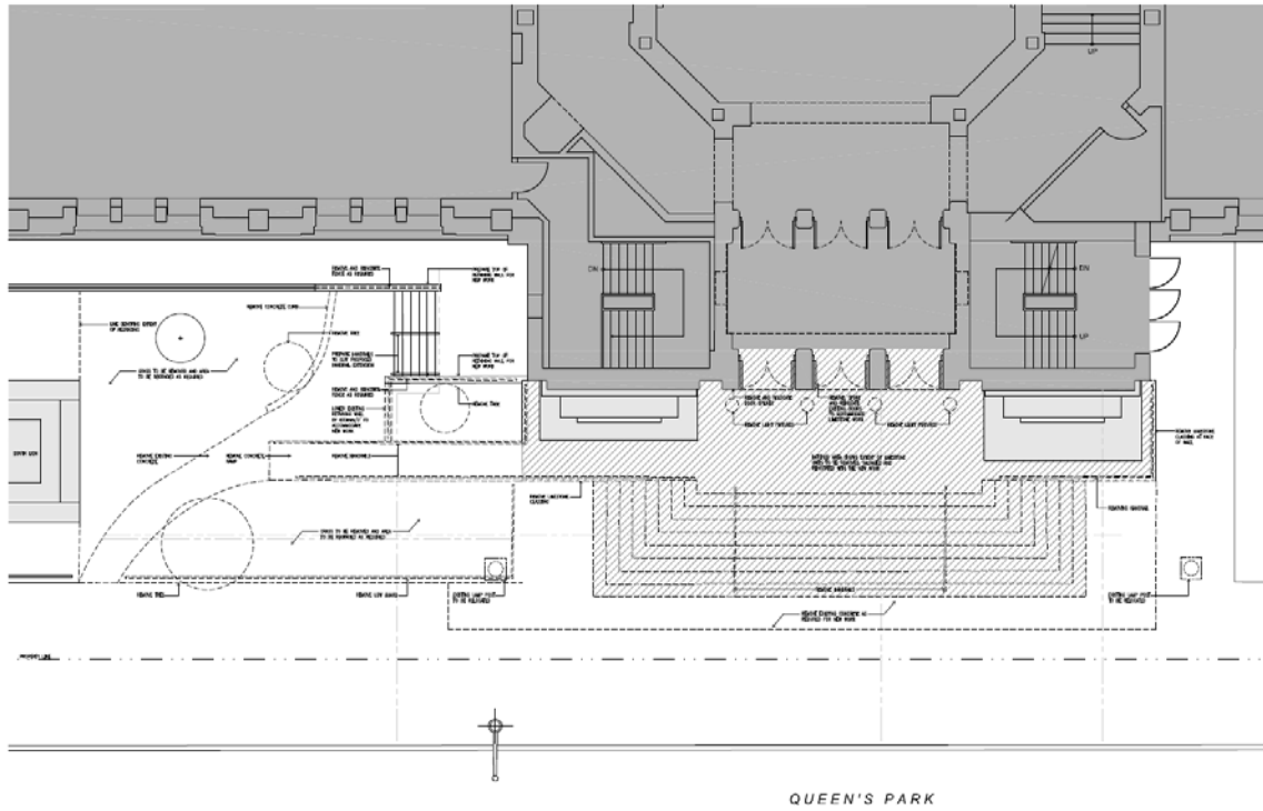
Demolition Plan
