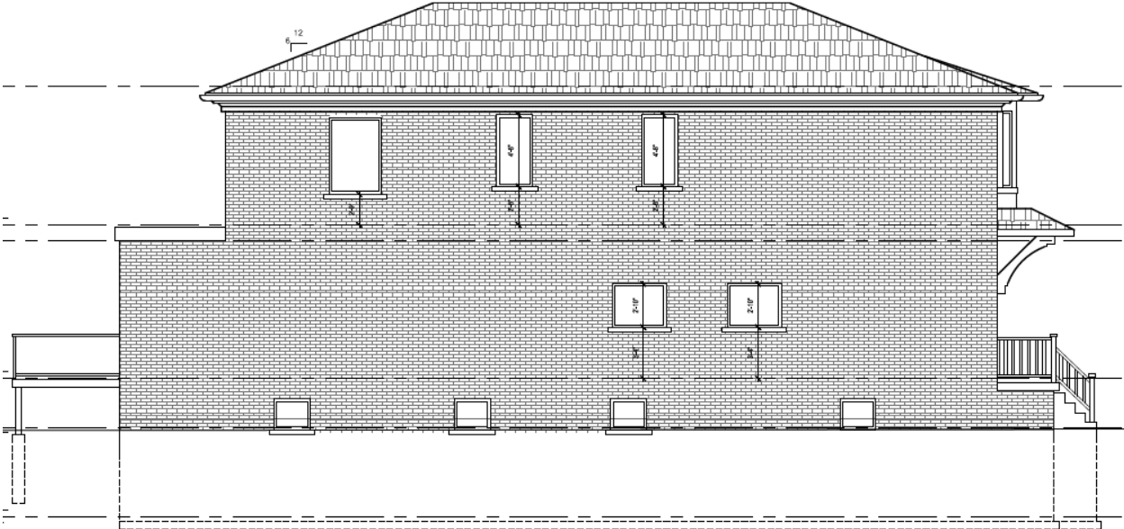
Proposed Side (East) Elevation
