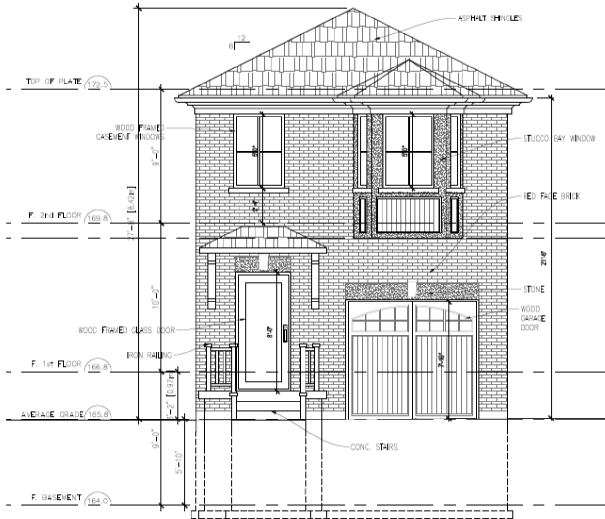
Proposed North (Front) Elevation
