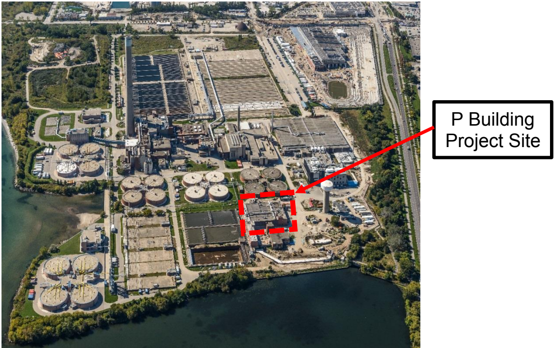
a) Aerial Photo of the Ashbridges Bay Treatment Plant – Showing Location of P Building
