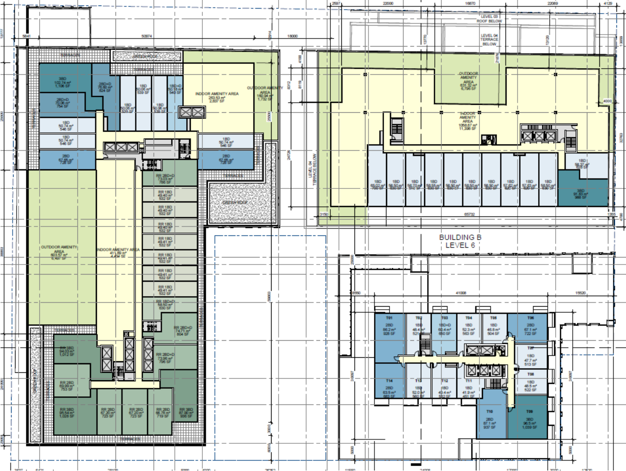
Proposed Sixth Floor Plan
