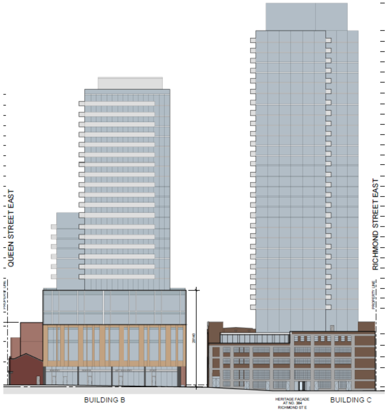
Proposed West Elevation (interior of site)
