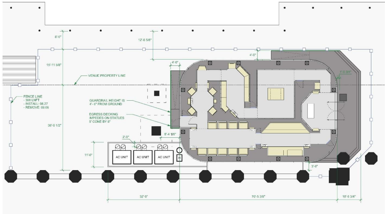
SITE PLAN
