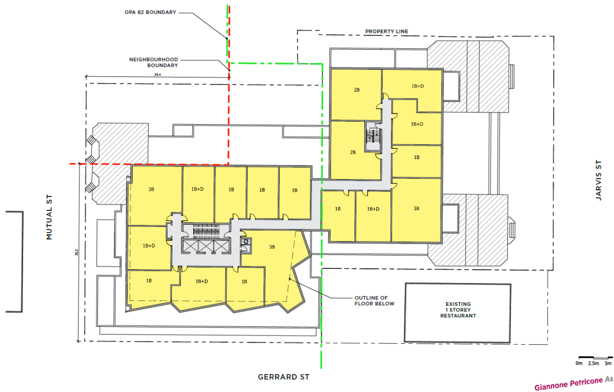
5 th -9 th floor plan
