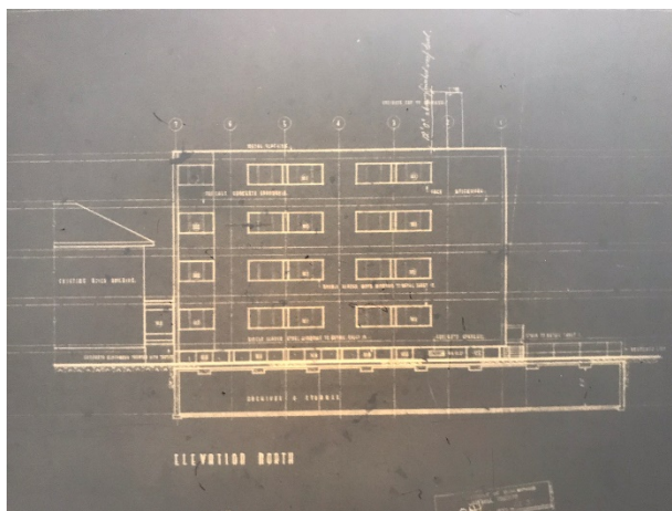
7b & c. Original 1959 architectural drawings of the Peter Dickinson-designed 4-storey rear addition at 226 St. George Street (now demolished), showing the north (at left) and south (at right) elevations. (City of Toronto Building Records File 54764)
