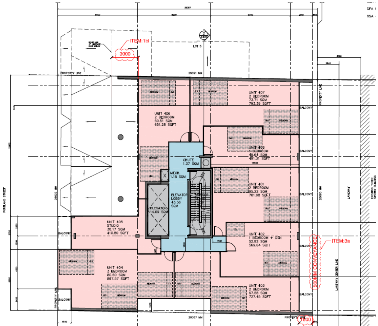
Floor 4 Plans
