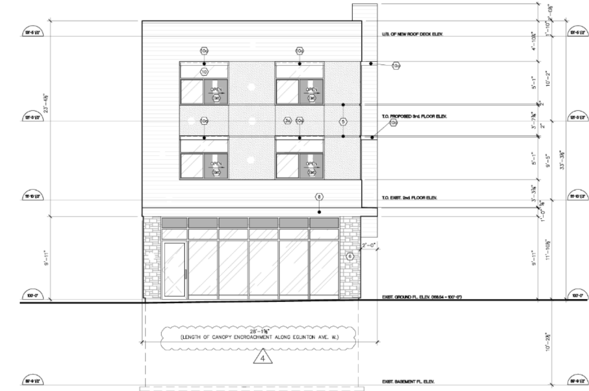
2 SOUTH ELEVATION A-4 1/4"=1'-0"
