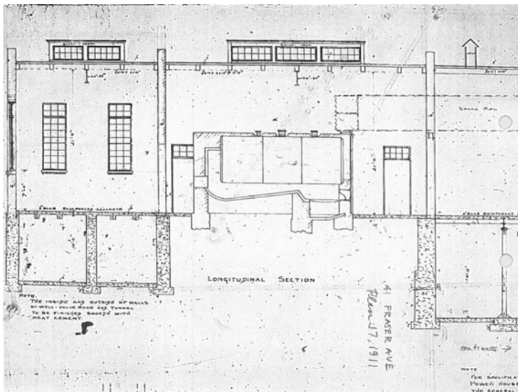
35. Longitudinal Section Drawing for the powerhouse, 1911(Building Records, Plan J7)
