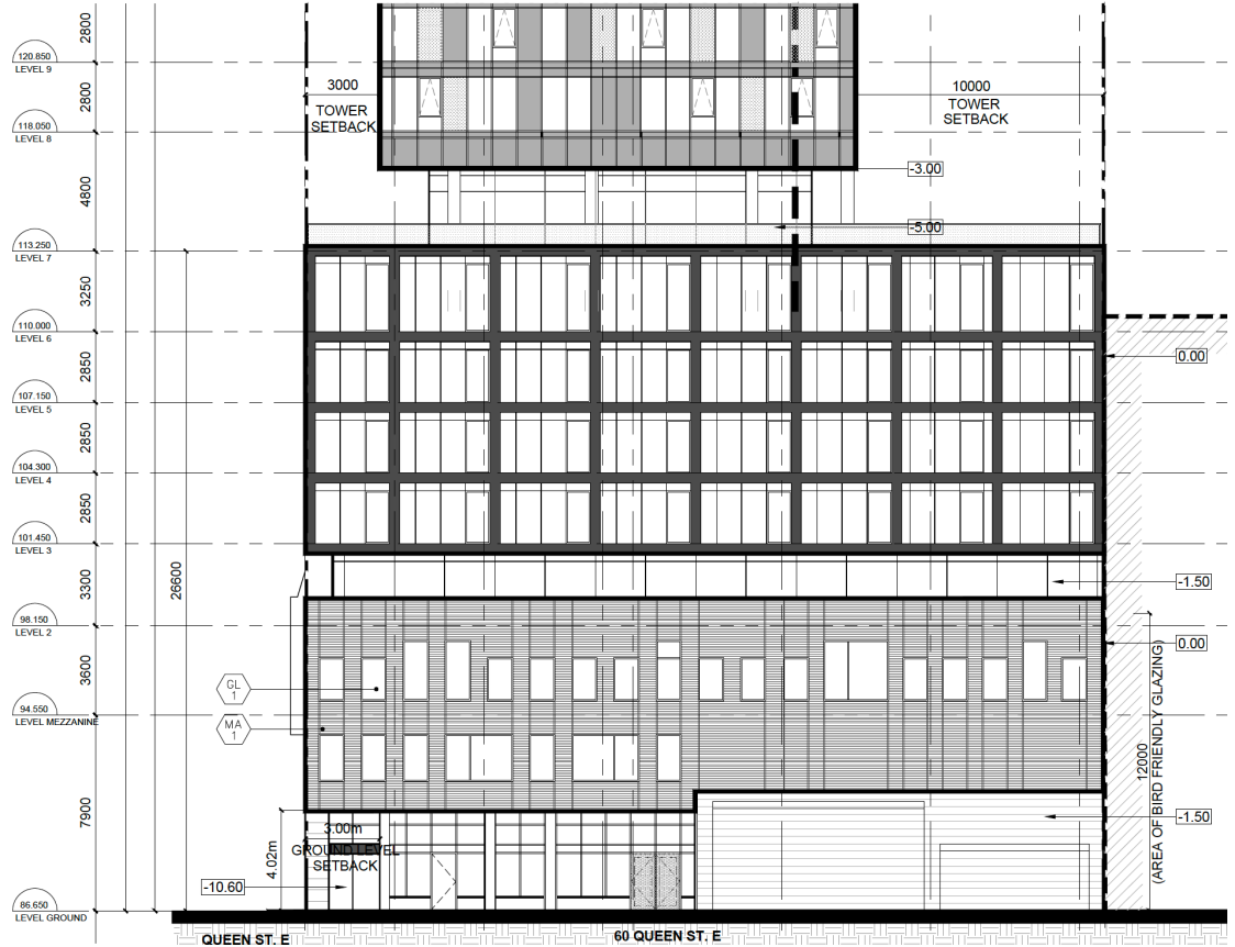
Dalhousie Street elevation
