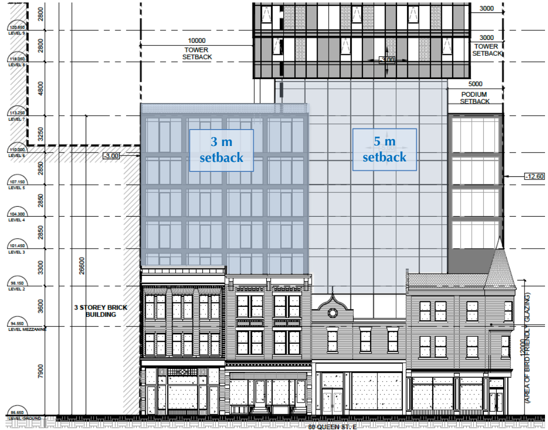
Church Street elevation
