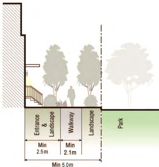
Figure 30 Cross-section of 5.0m Required Setback Area
