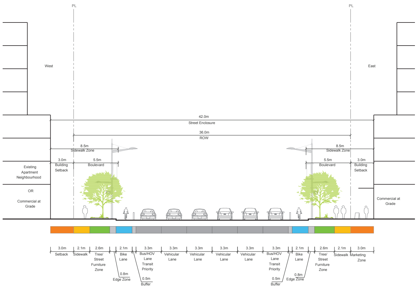
Figure 10 Conceptual Cross-section of Widened Victoria Park Avenue and Warden Avenue (36m ROW)
