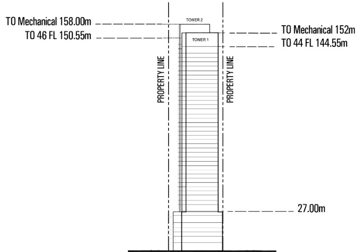
West Elevation
