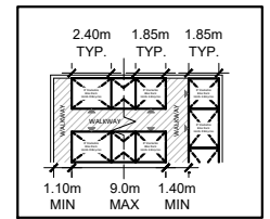
TYPICAL BICYCLE PARKING DIMENSIONS
