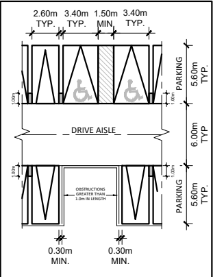
TYPICAL VEHICULAR PARKING DIMENSIONS
