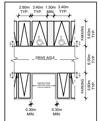
TYPICAL VEHICULAR PARKING DIMENSIONS
