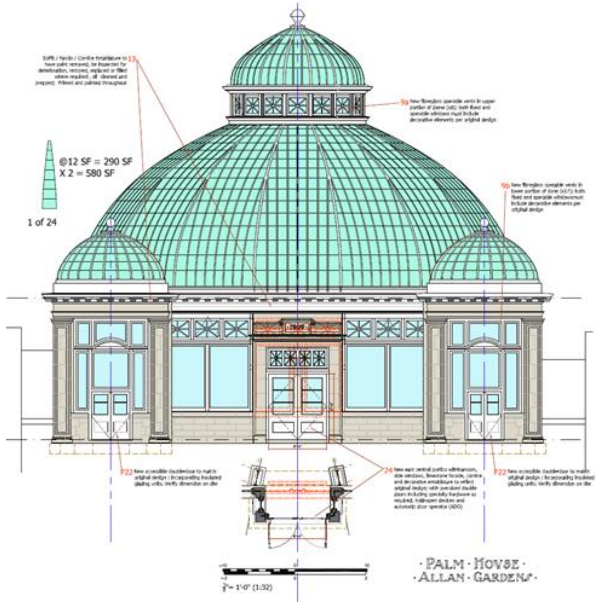
East Elevation Drawing
