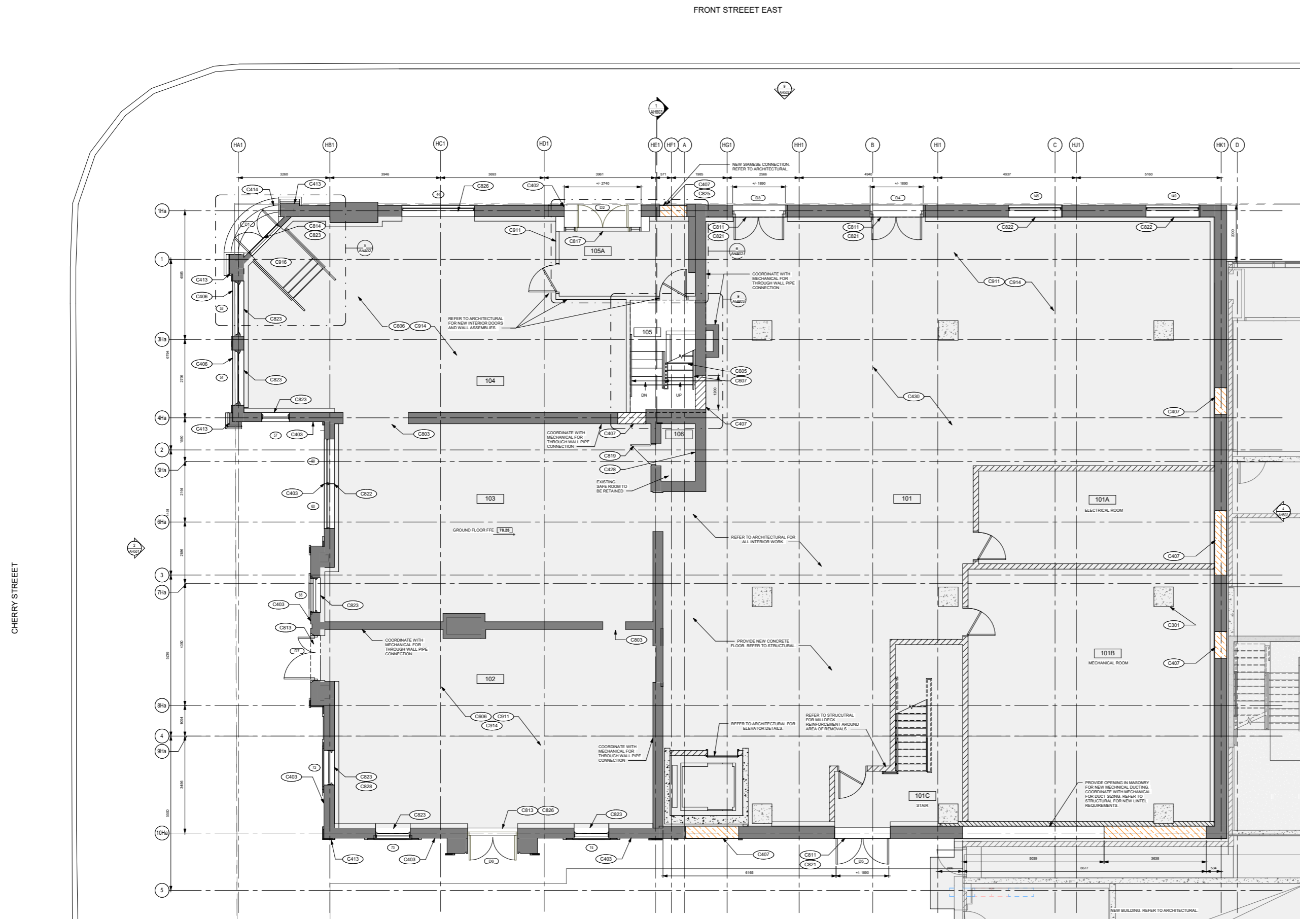
Ground floor plan. ERA
