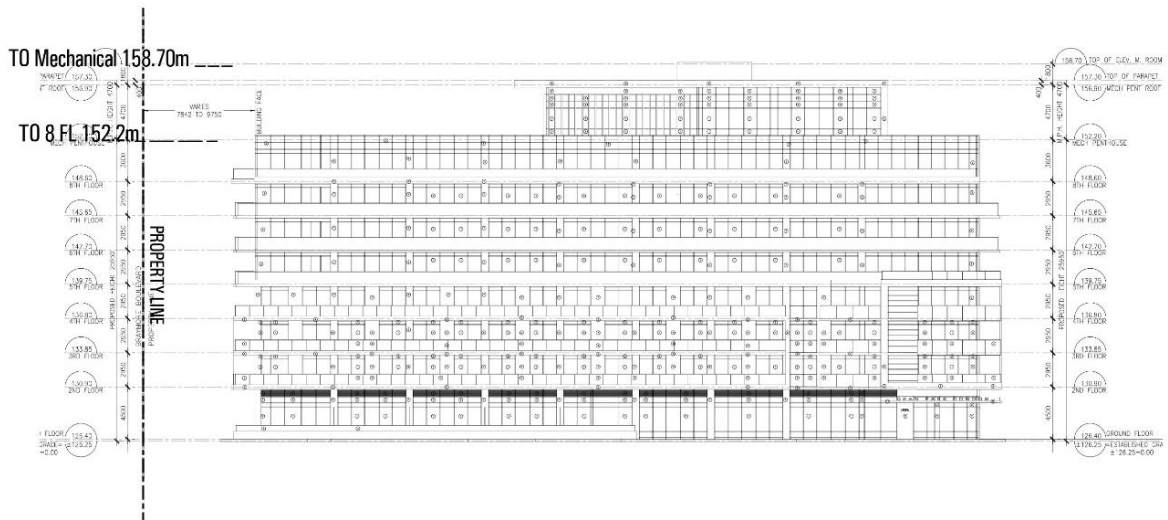
Building A South Elevation
