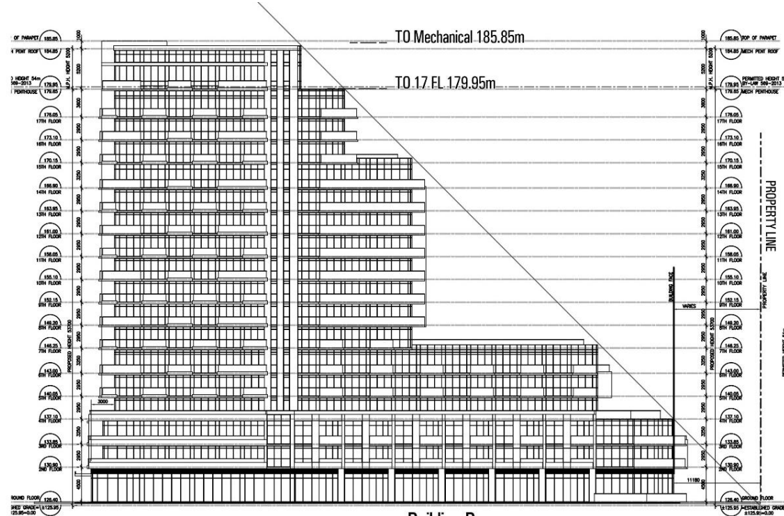
Building B East Elevation
