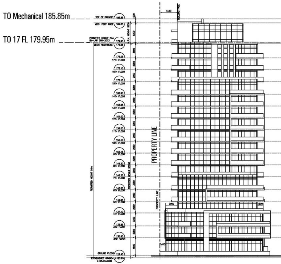
Building B South Elevation
