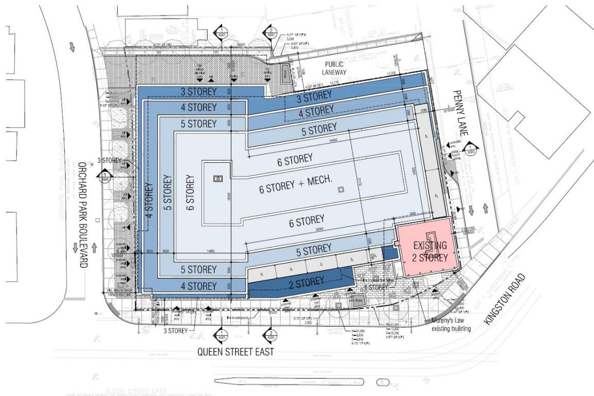
Site Plan
