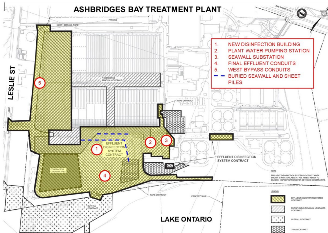
Figure 1 – Site Plan of Disinfection Project
