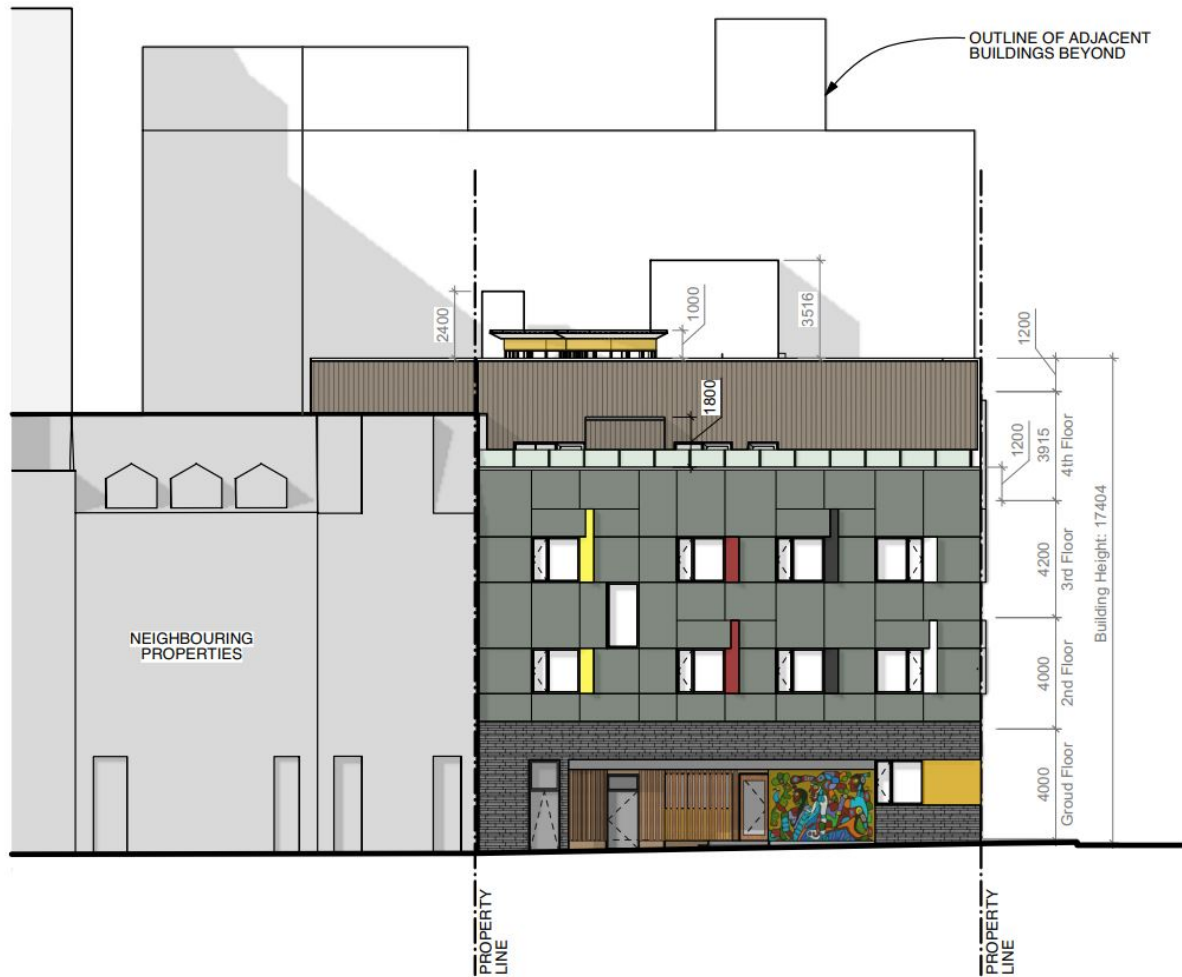
East Elevation (Hilditch Architect Inc., May 14, 2021)
