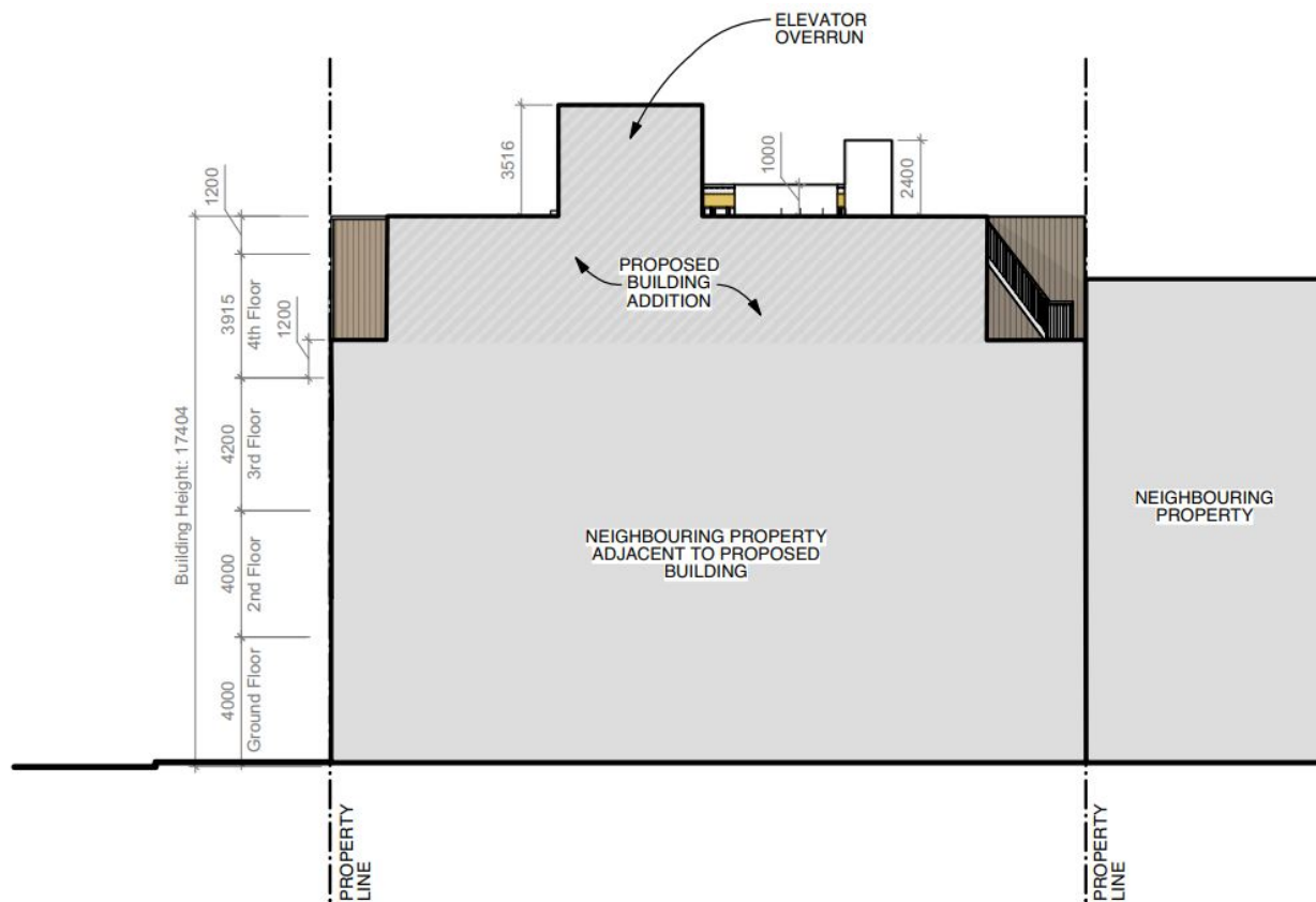
West Elevation (Hilditch Architect Inc., May 14, 2021)
