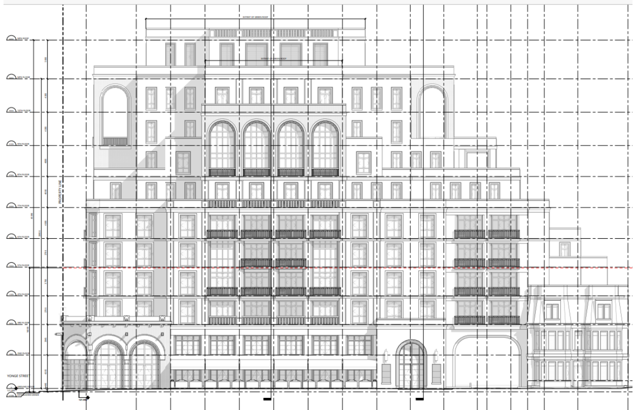
North Façade
