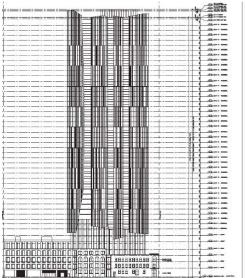
South Elevation
