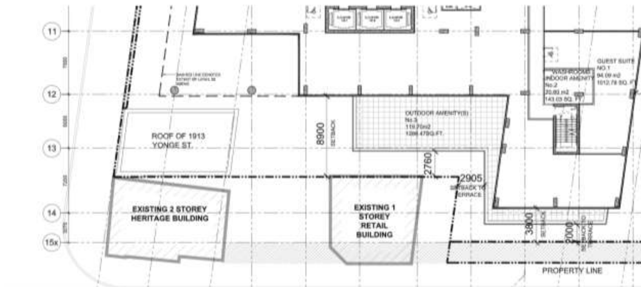
Extract from Level 2 Floor Plan showing no development on the roof of 1913 Yonge Street.
