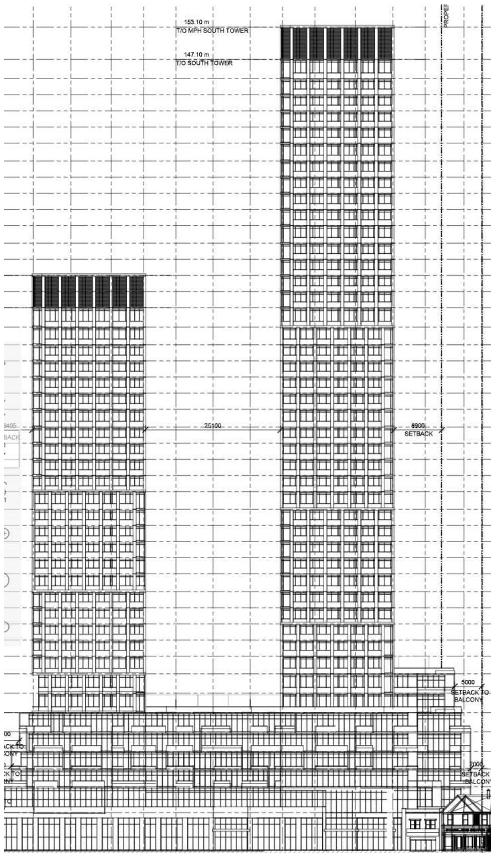
West Elevation at Yonge Street.
