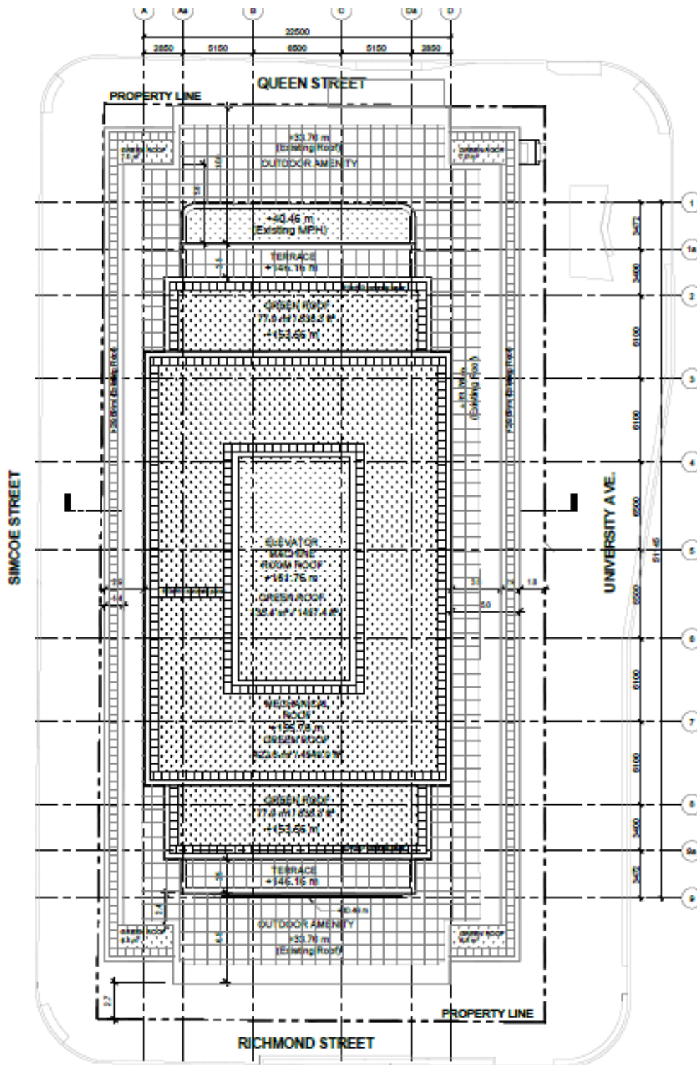
250 University Avenue - Roof Plan. For the complete drawing set, please visit the Application Information Centre.
