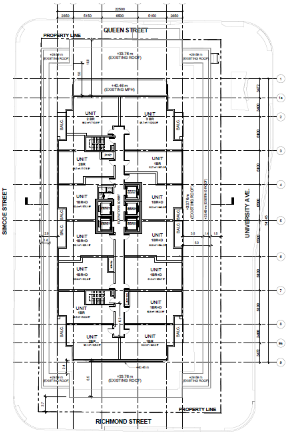
250 University Avenue - Typical Floor Plan, lower tower (above heritage property). For the complete drawing set, please visit the Application Information Centre .
