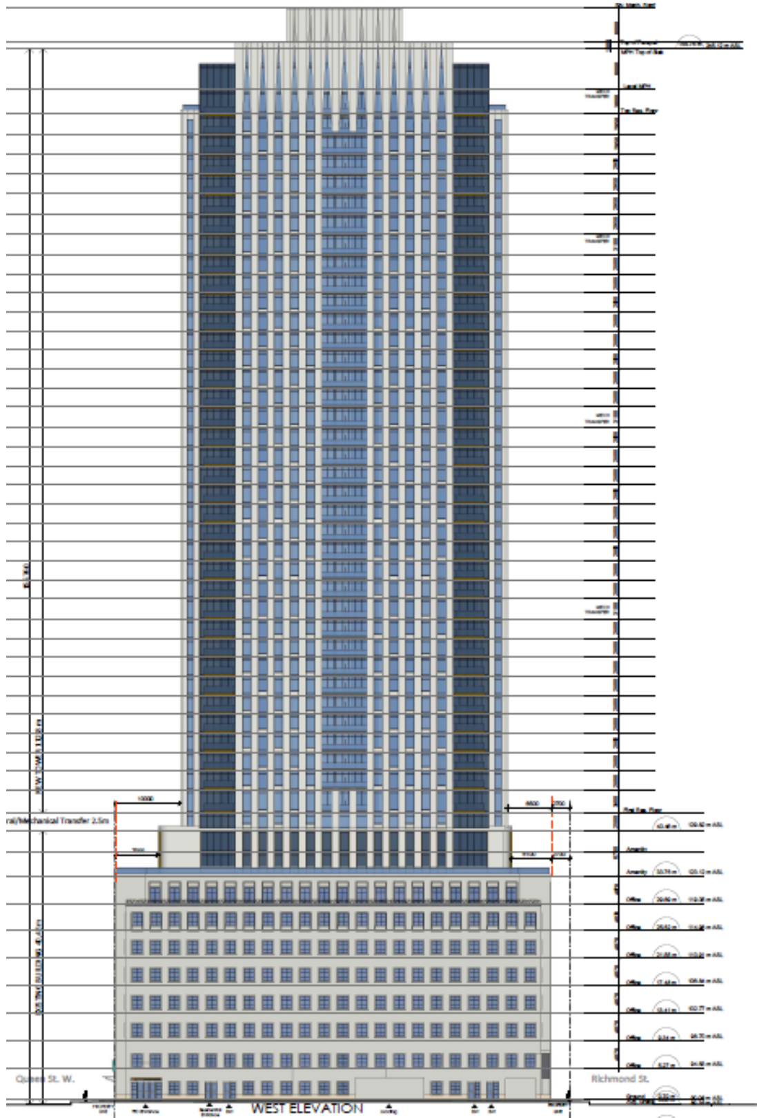
West Elevation at Simcoe Street. For the complete drawing set, please visit the Application Information Centre .
