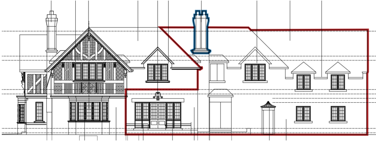
Existing south elevation with red outline area indicating portion of house to be removed. (Source: Wayne Swadron Architects, 2022)
