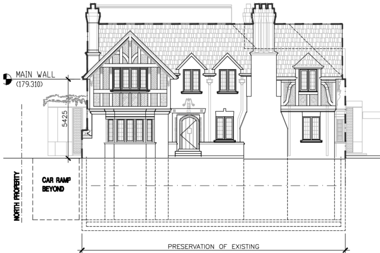
Primary (west) elevation (Source: Hariri Pontarini Architects, 2022).
