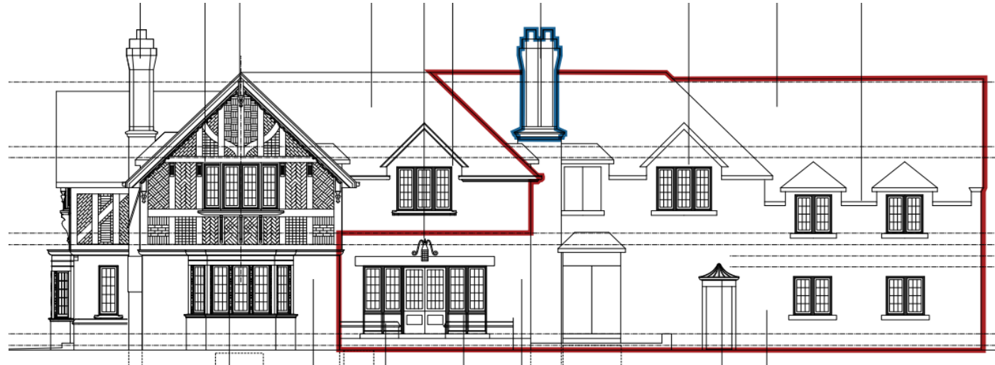
Existing south elevation with area outlined in red showing portion of house to be removed. (Source: Wayne Swadron Architects, 2022)
