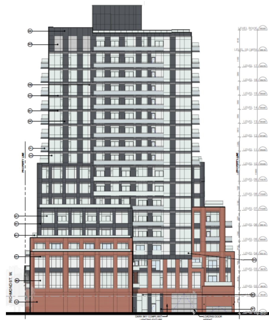
Proposed West Elevation
