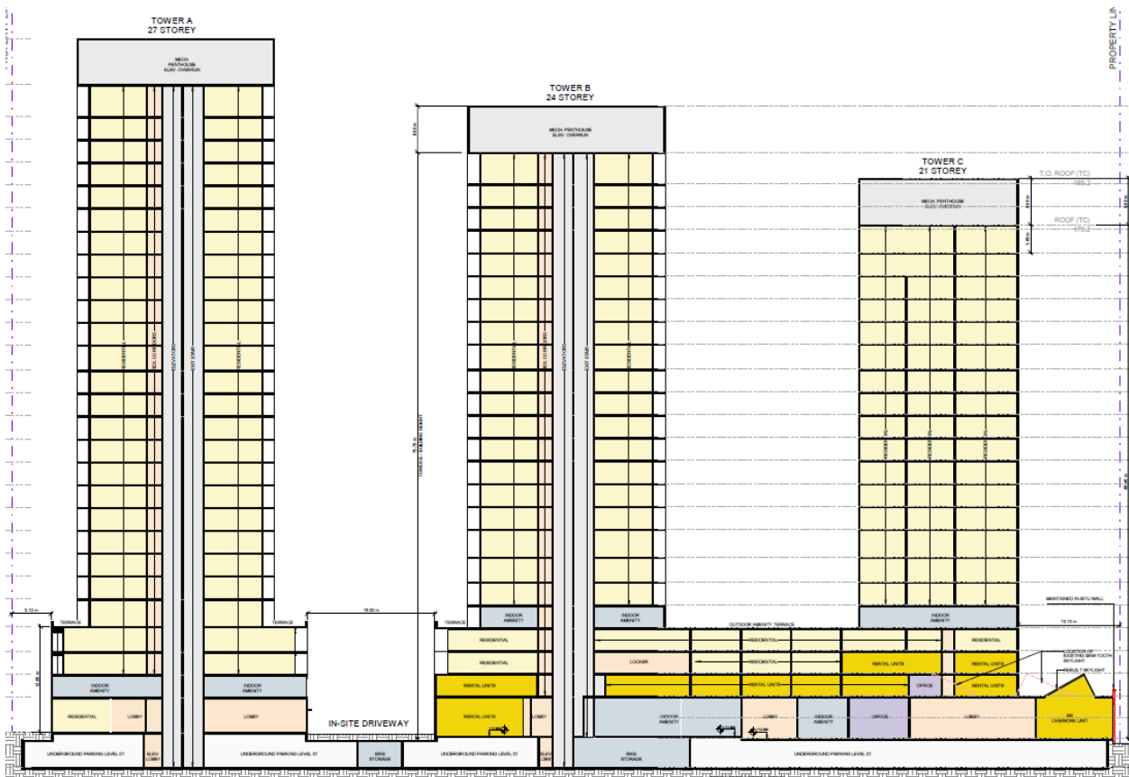
Proposed Building Section (Turner Fleisher Architects Inc.,)
