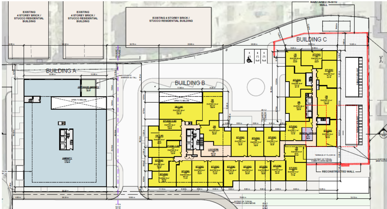
Proposed Second Floor Plan with retained facades noted in red (Turner Fleisher Architects Inc.,)
