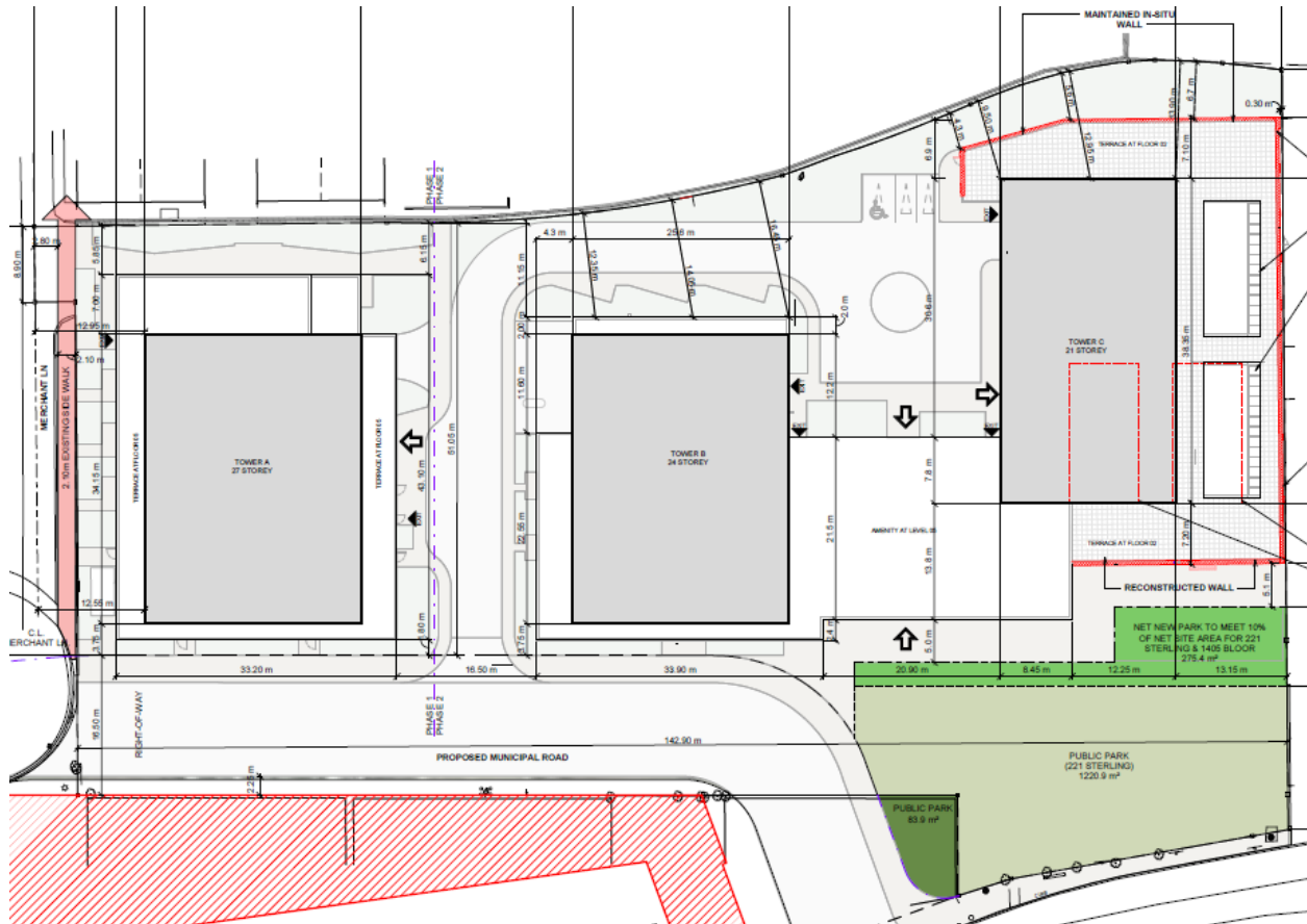
Proposed Site Plan with retained facades noted in red (Turner Fleisher Architects Inc.,)
