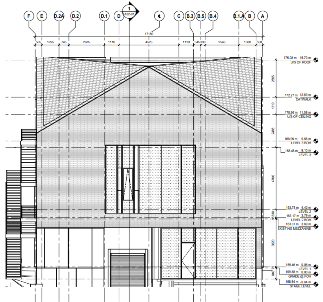
Proposed rear (east) elevation of 551 Mount Pleasant Road (NORR/Hariri Pontarini Architects, 2022)
