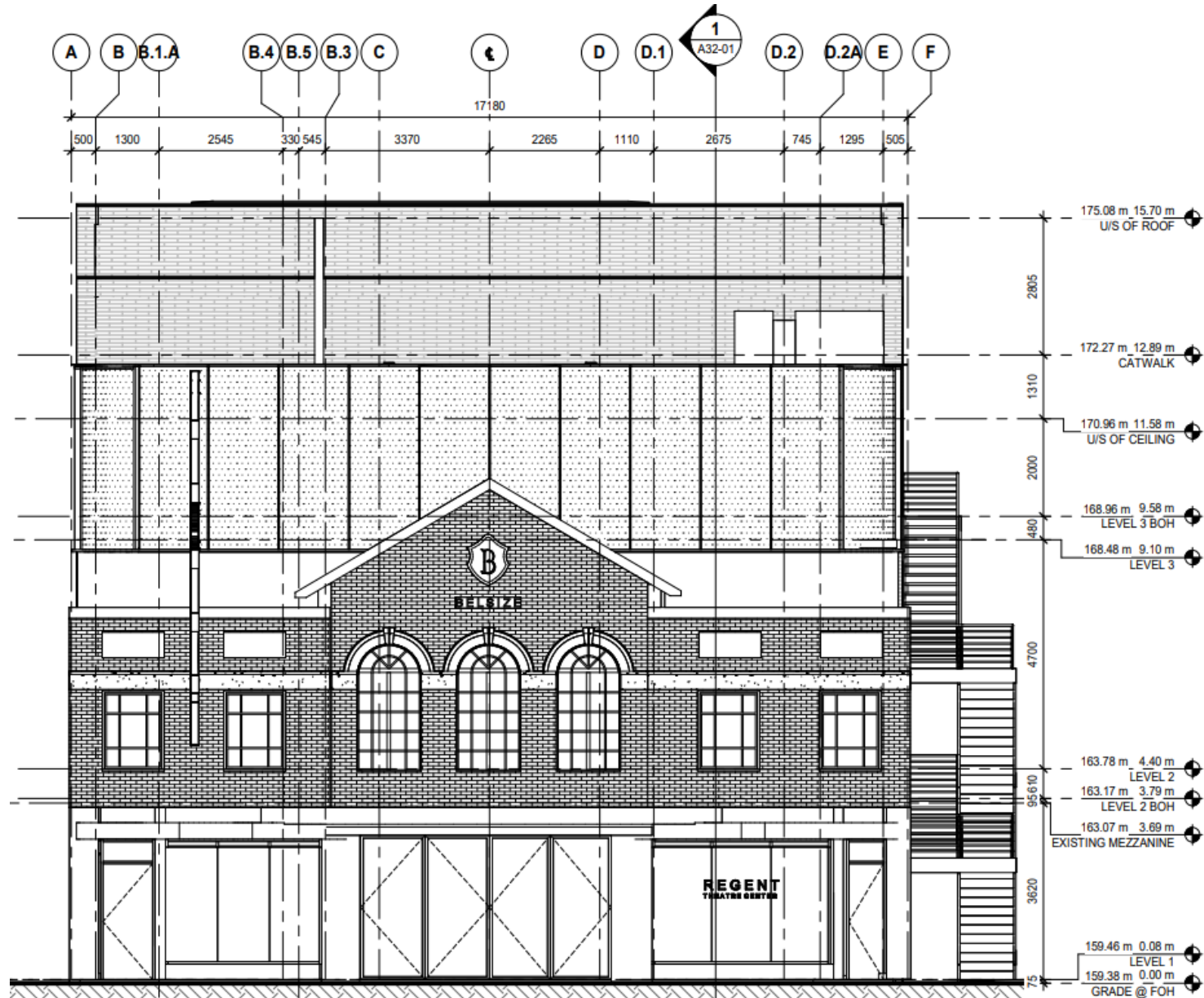
Proposed principal (west) elevation of 551 Mount Pleasant Road (NORR/Hariri Pontarini Architects, 2022)
