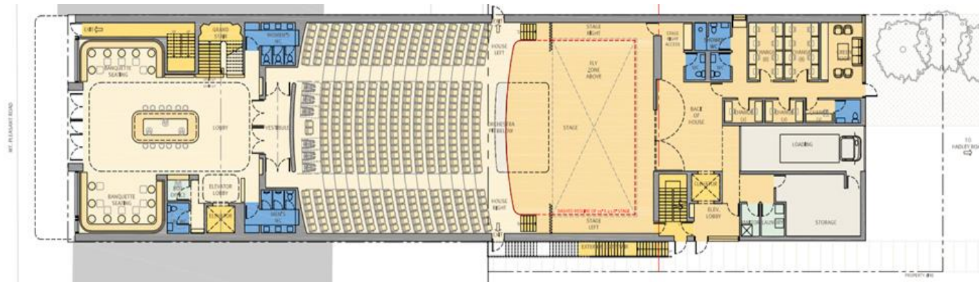
Proposed ground floor of 551 Mount Pleasant Road (NORR/Hariri Pontarini Architects, 2022)
