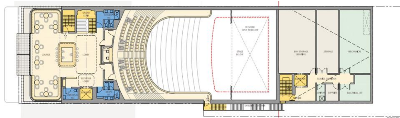
Proposed third floor of 551 Mount Pleasant Road (NORR/Hariri Pontarini Architects, 2022)
