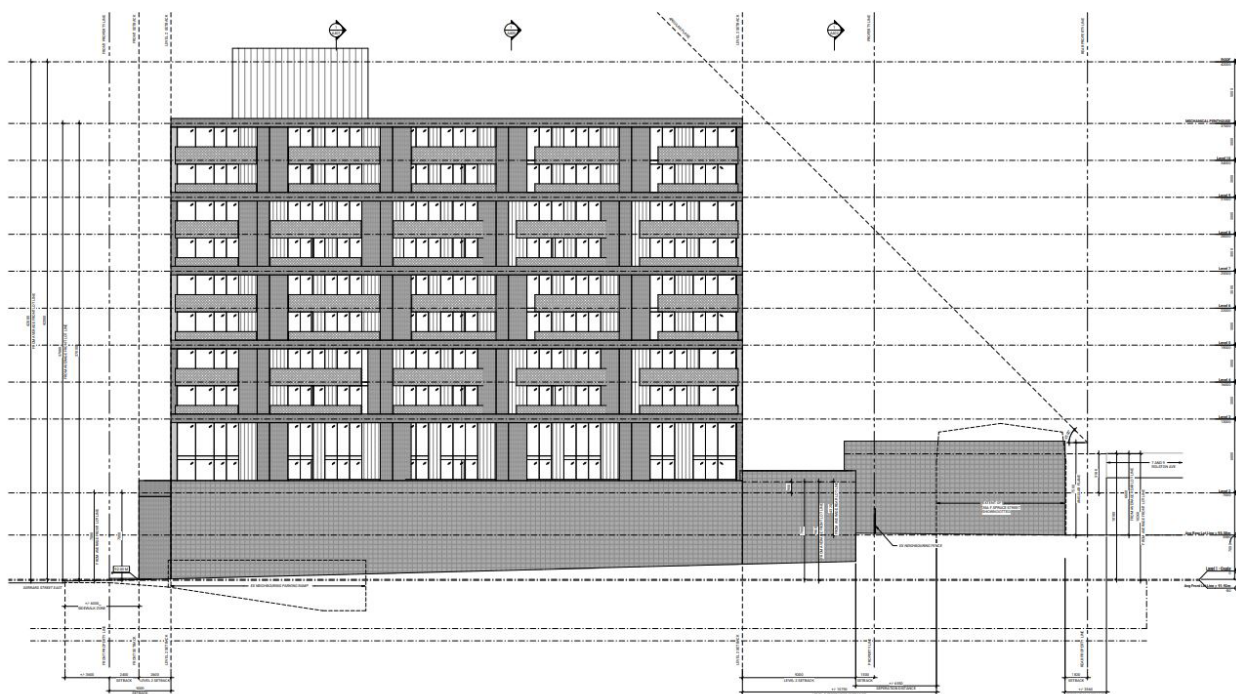
East elevation drawing (Diamond Schmitt Architects, January 27, 2023)
