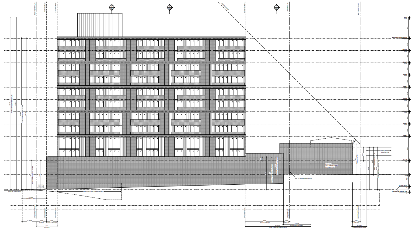
Drawing of east elevation (Diamond Schmitt Architects, September 21, 2023)
