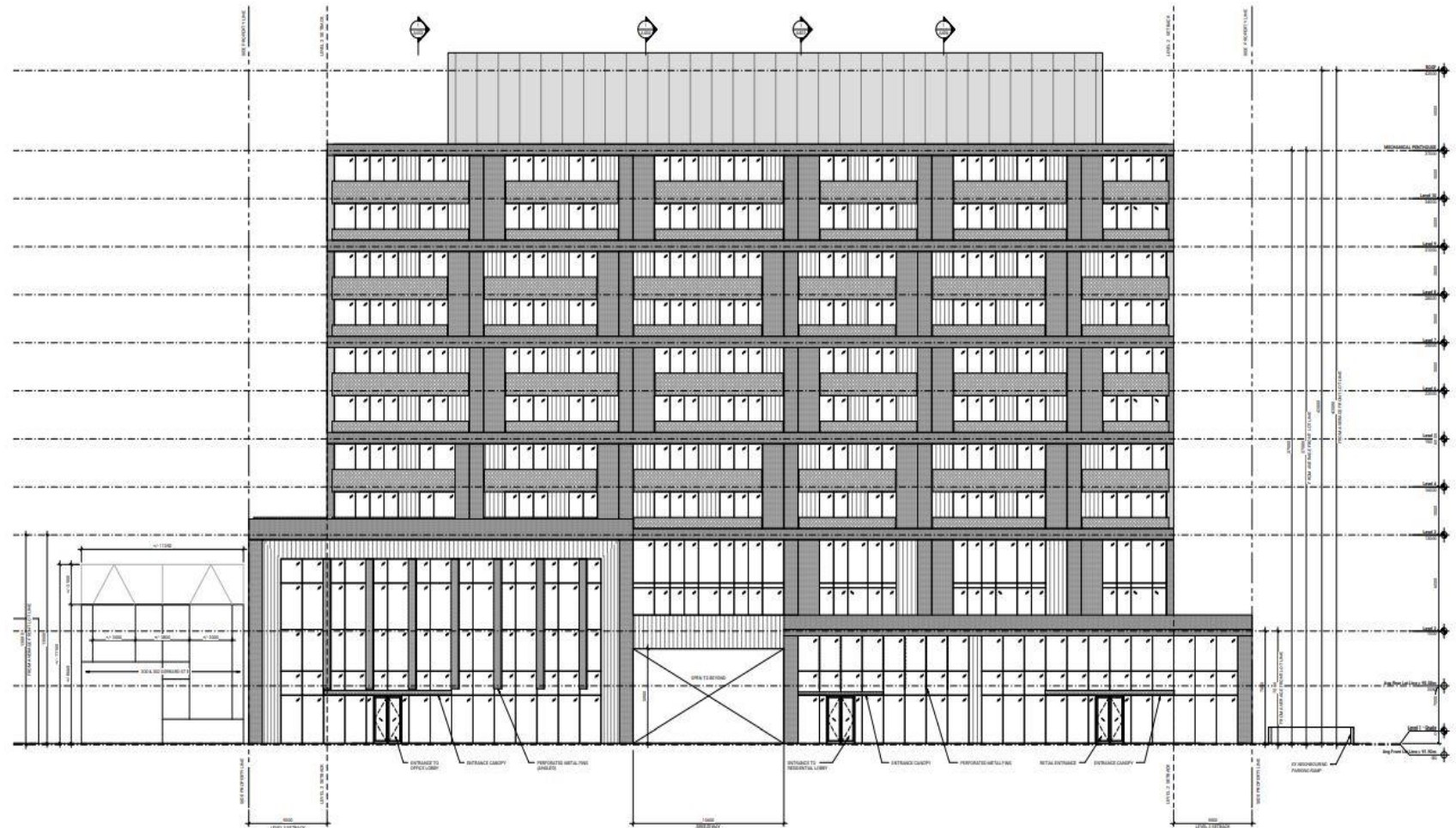
South elevation drawing (Diamond Schmitt Architects, January 27, 2023)
