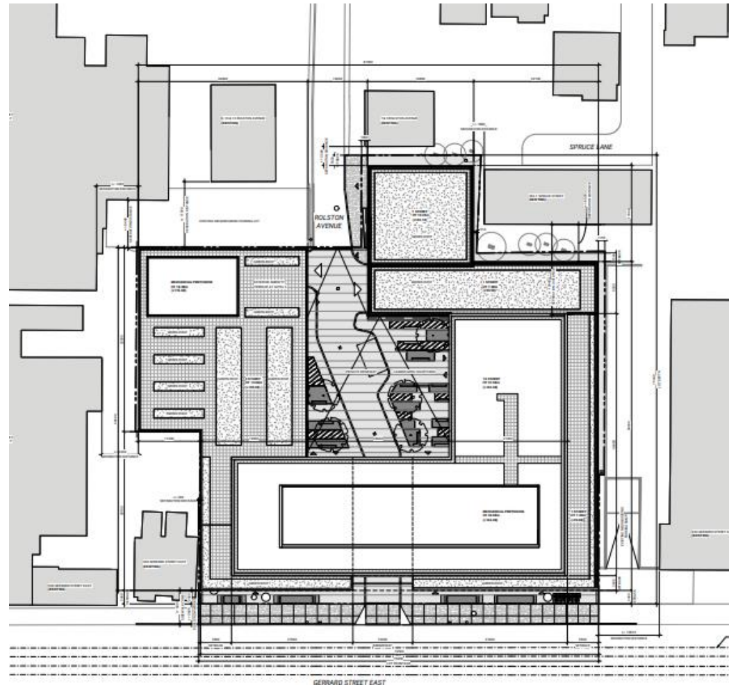
Site plan (Diamond Schmitt Architects, September 21, 2023)
