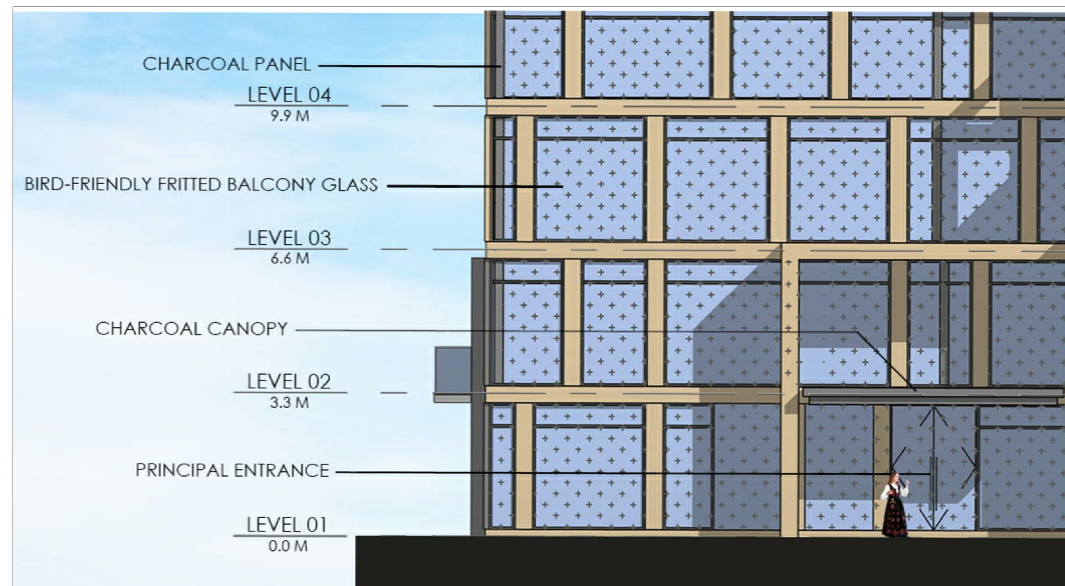
5. BLOCK 5 - MAIN ENTRANCE
