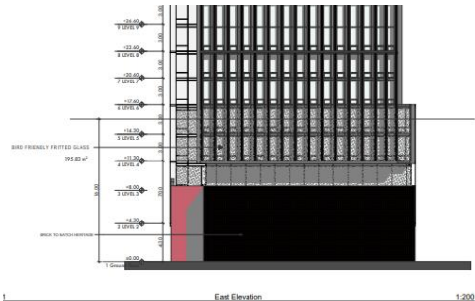
East Elevation - East Return Wall of Heritage Property at Lower left of Diagram
