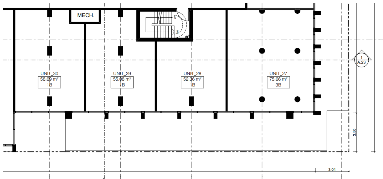
Floors Four and above. 3.5 Metre Stepback from Front Façade at King Street West
