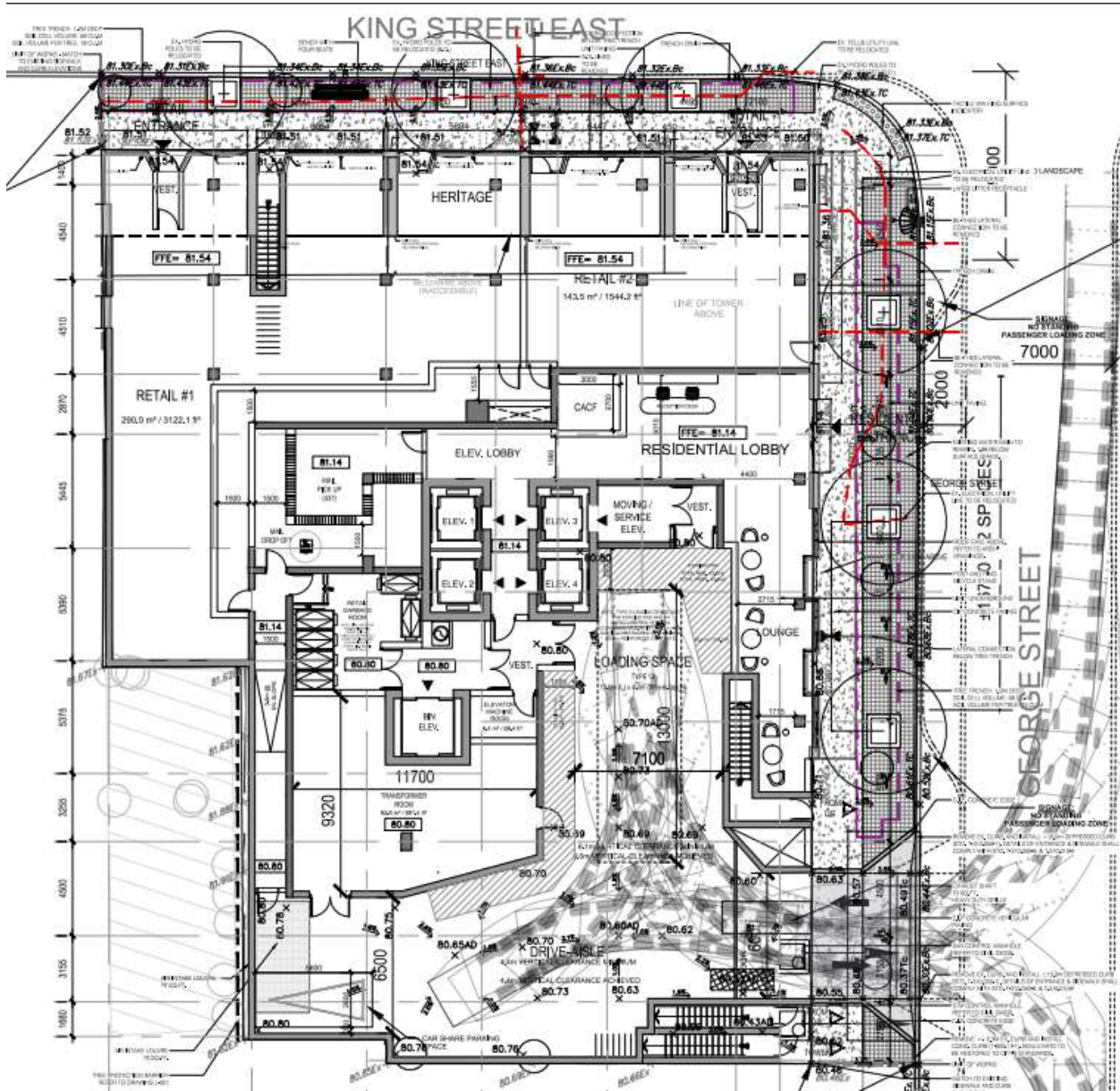
Proposed ground floor plan for 175-185 King Street East included for illustration purposes (IBI Group/Arcadis, 2024).
