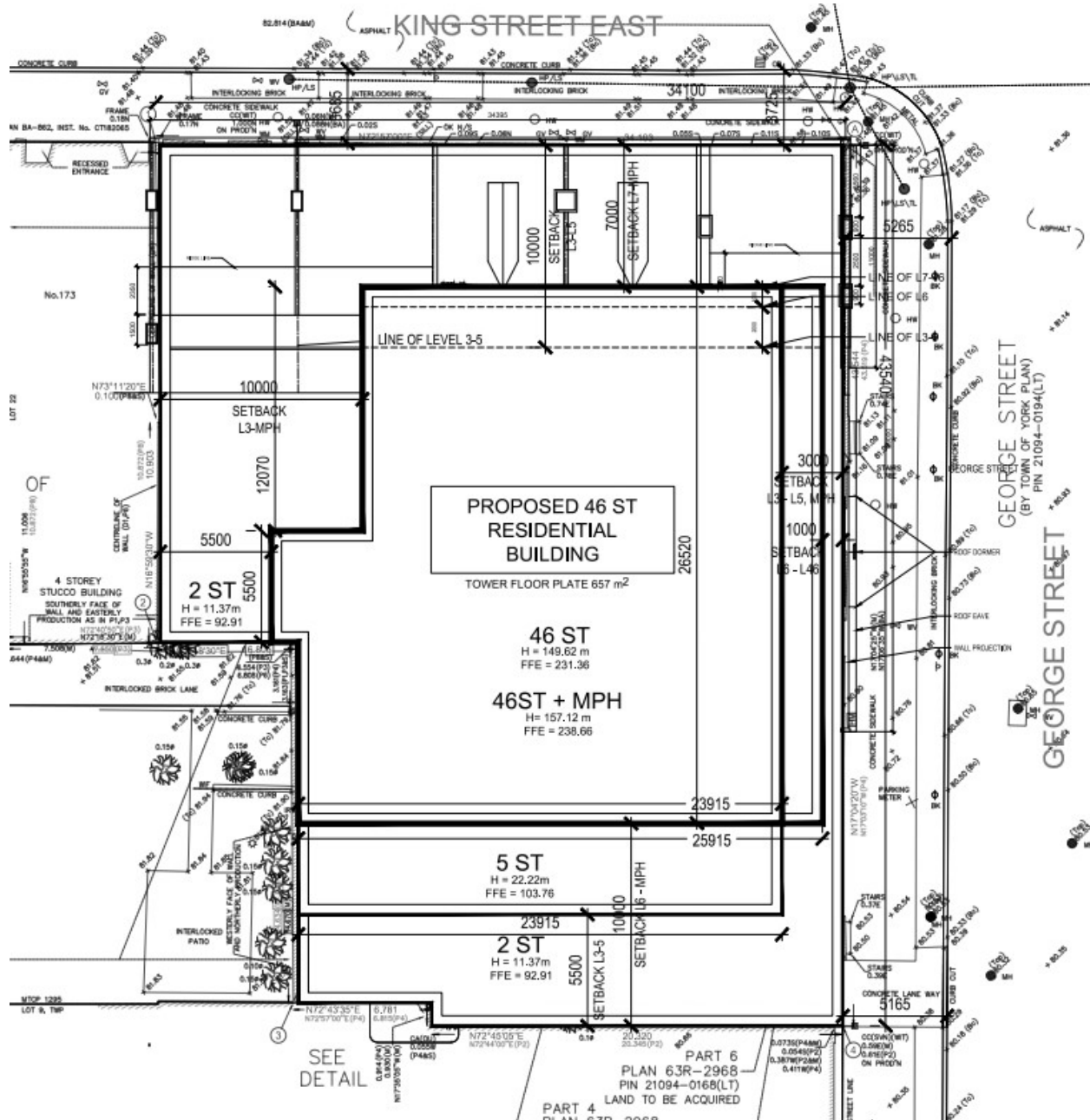
Proposed site plan for 175-185 King Street East included for illustration purposes (IBI Group/Arcadis, 2024).
