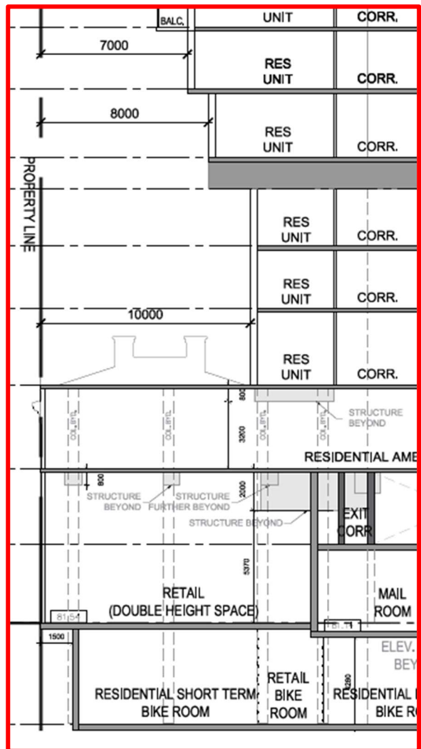
Proposed east-west cross-section drawings for 175-185 King Street East included for illustration purposes (IBI Group/Arcadis, 2024).
