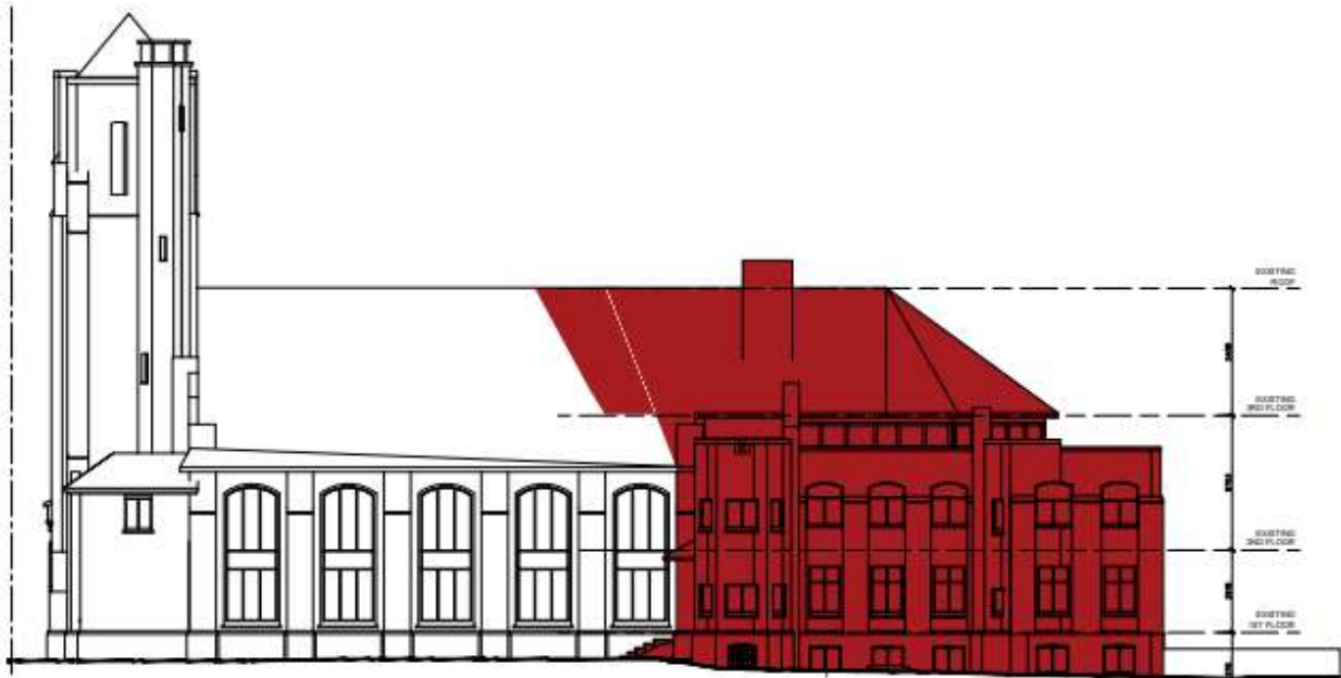
Drawing of the south elevation of 415 Broadview Avenue, showing the proposed portions to be removed in red, included for illustration purposes (RAW Design Inc., 2024, annotated by ERA Architects Inc., 2024).
