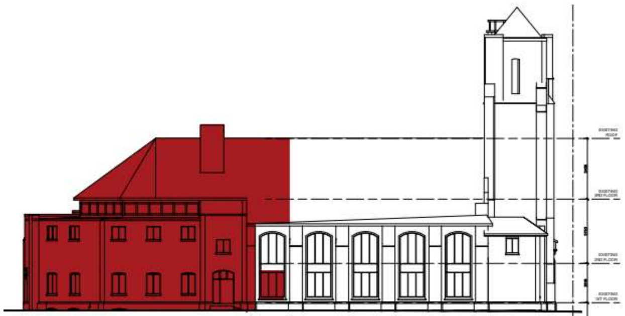
Drawing of the north elevation of 415 Broadview Avenue, showing the proposed portions to be removed in red, included for illustration purposes (RAW Design Inc., 2024, annotated by ERA Architects Inc., 2024).
