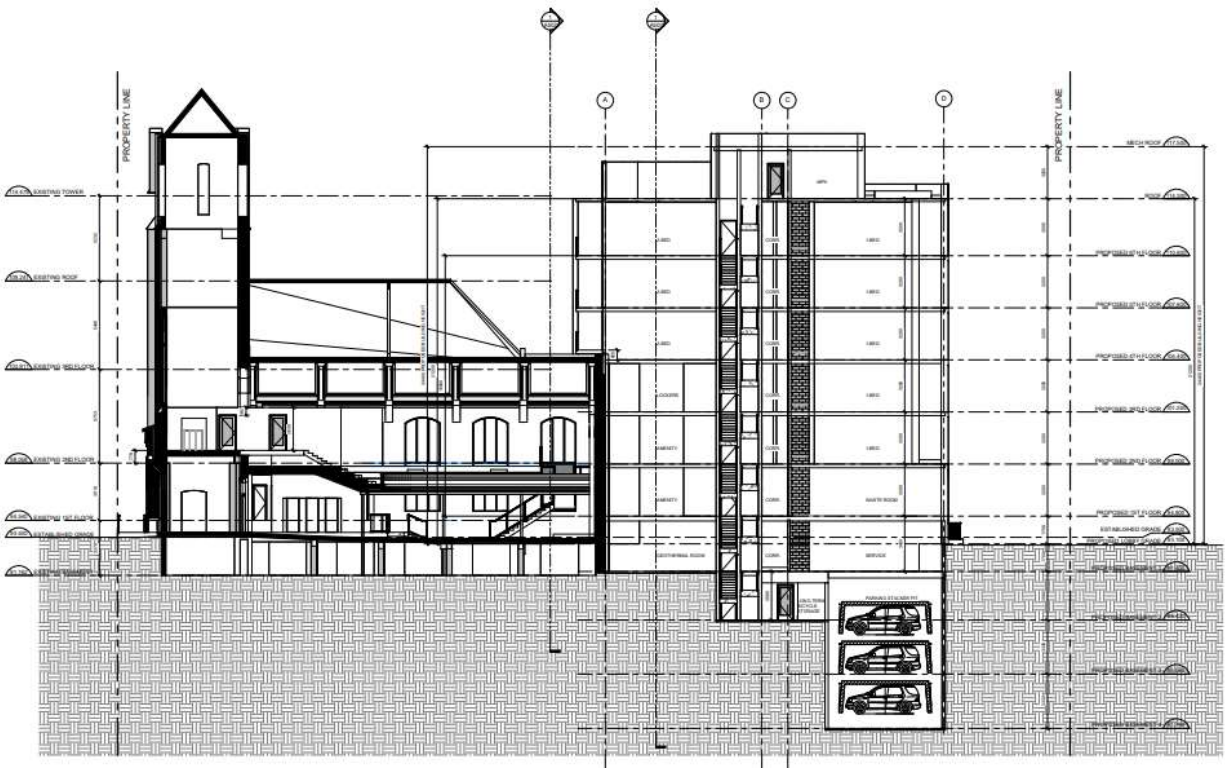
Proposed cross-section drawing for 415 Broadview Avenue included for illustration purposes (RAW Design Inc., 2024).
