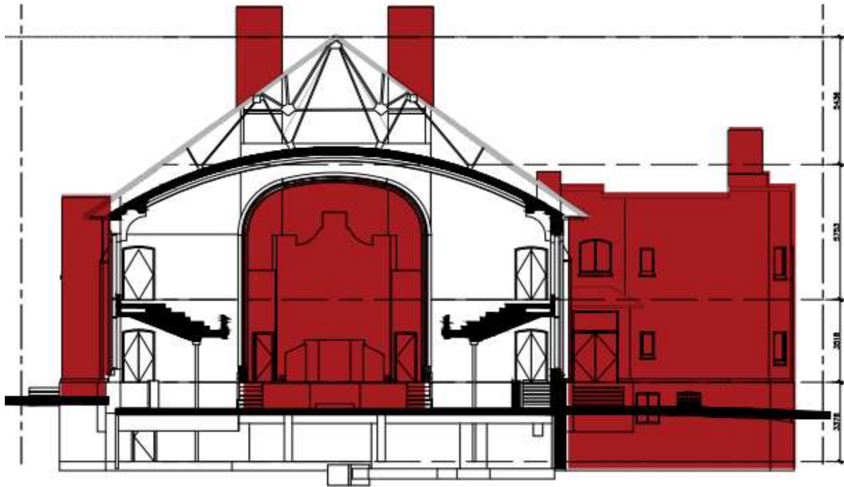
East-west cross section drawing of 415 Broadview Avenue, showing the proposed portions to be removed in red, included for illustration purposes (RAW Design Inc., 2024, annotated by ERA Architects Inc., 2024).
