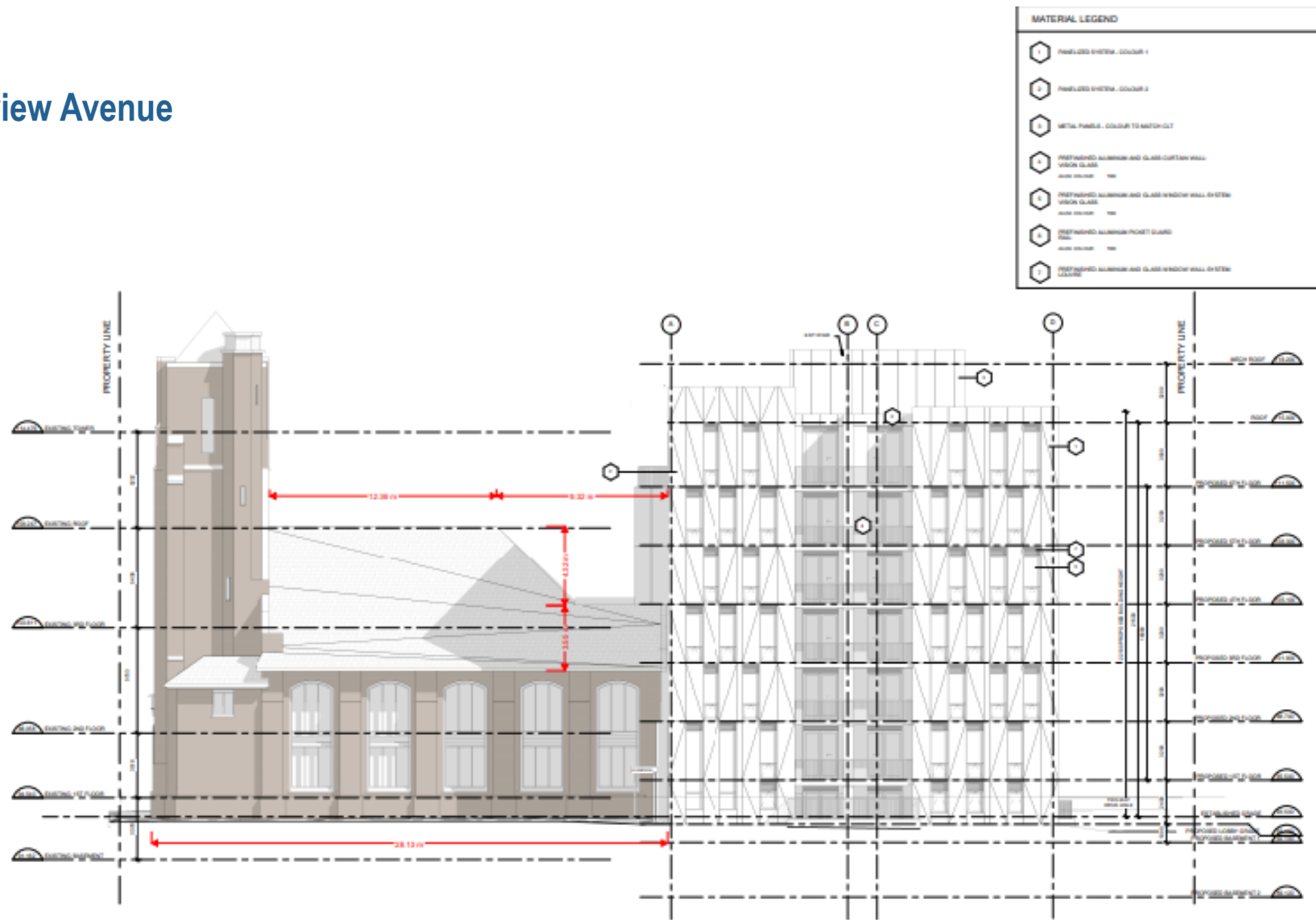
South elevation plan (RAW Design Inc., 2024, annotated by ERAArchitects Inc., 2024)
