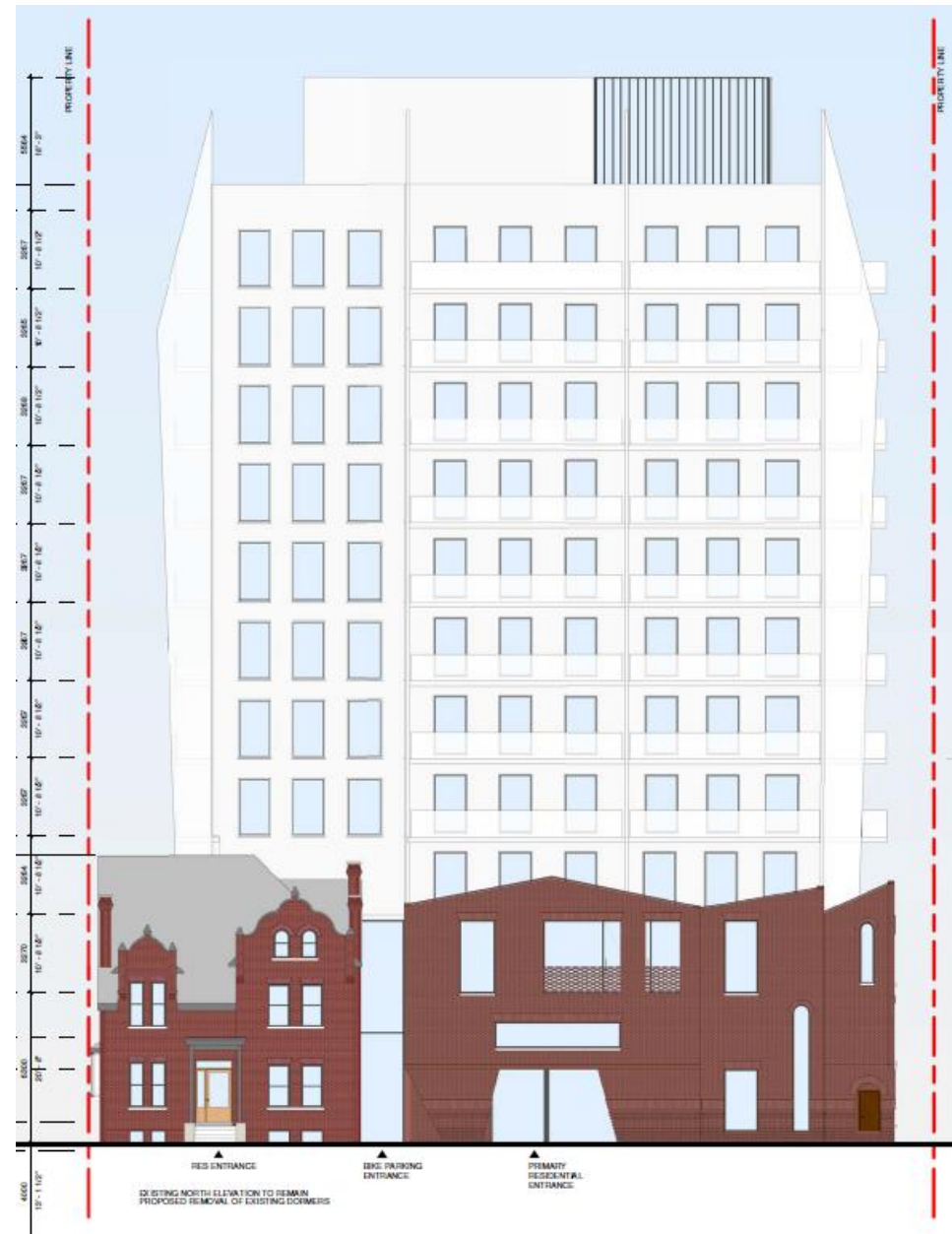
North Elevation (Gabriel Fain Architects Inc.)
